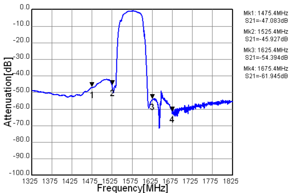
Fig.1 Pass-band Characteristics
