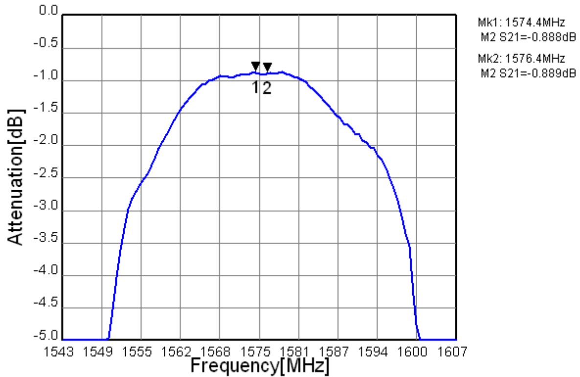
Fig.3 In-band Characteristics
