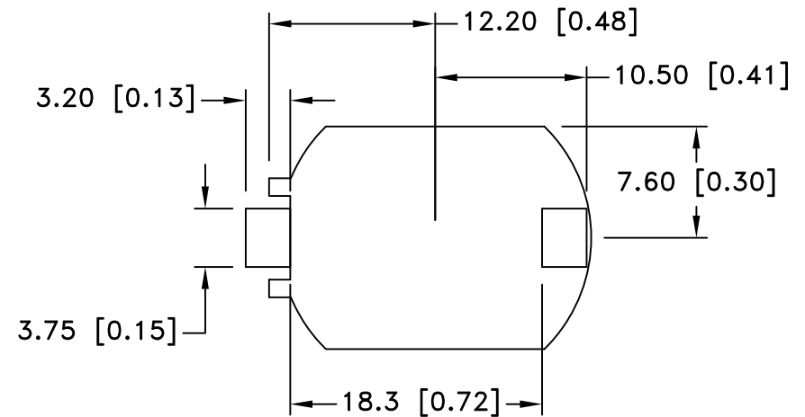
PCB LAYOUT
