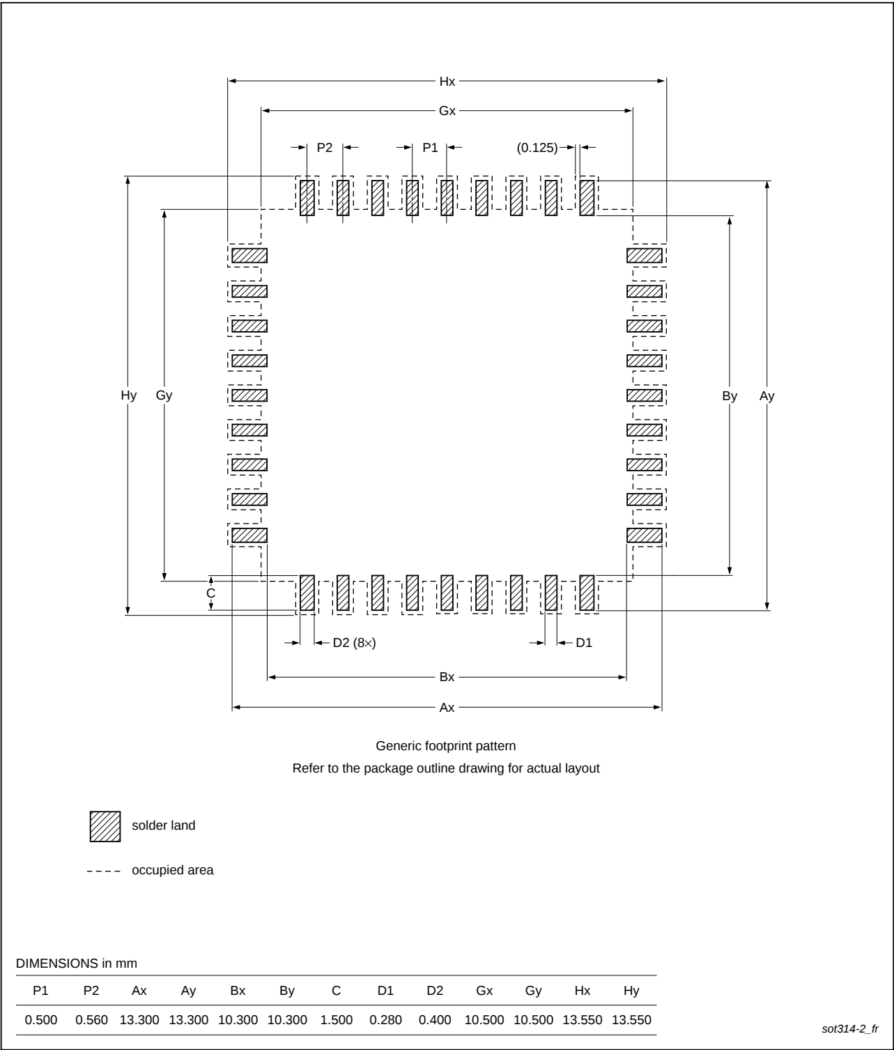
Fig 35. Reflow soldering for the LQFP64 package
