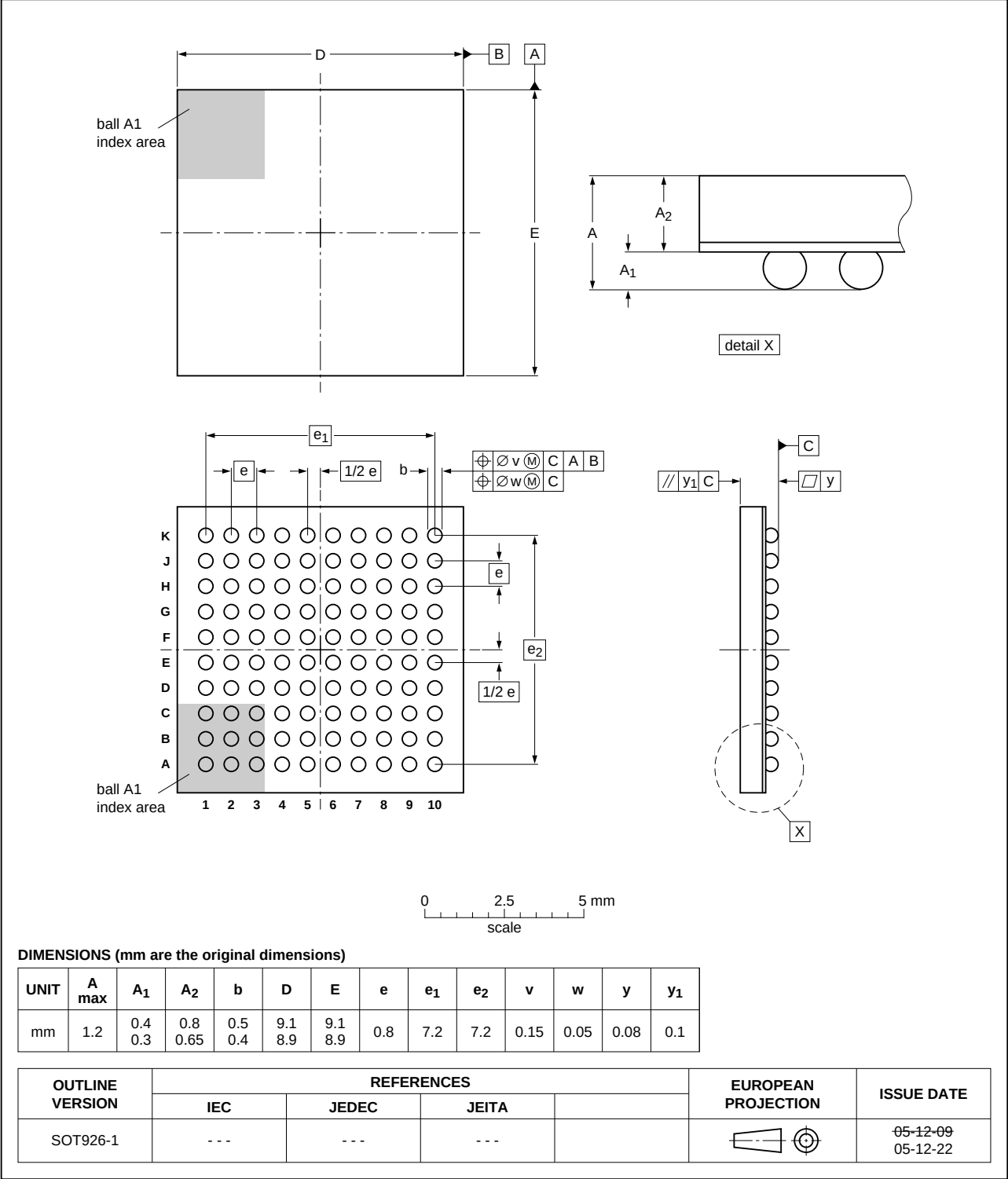
Fig 47. Package outline of the TFBGA100 package
