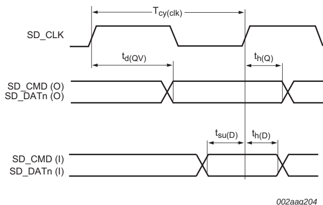
Fig 36. SD/MMC timing
