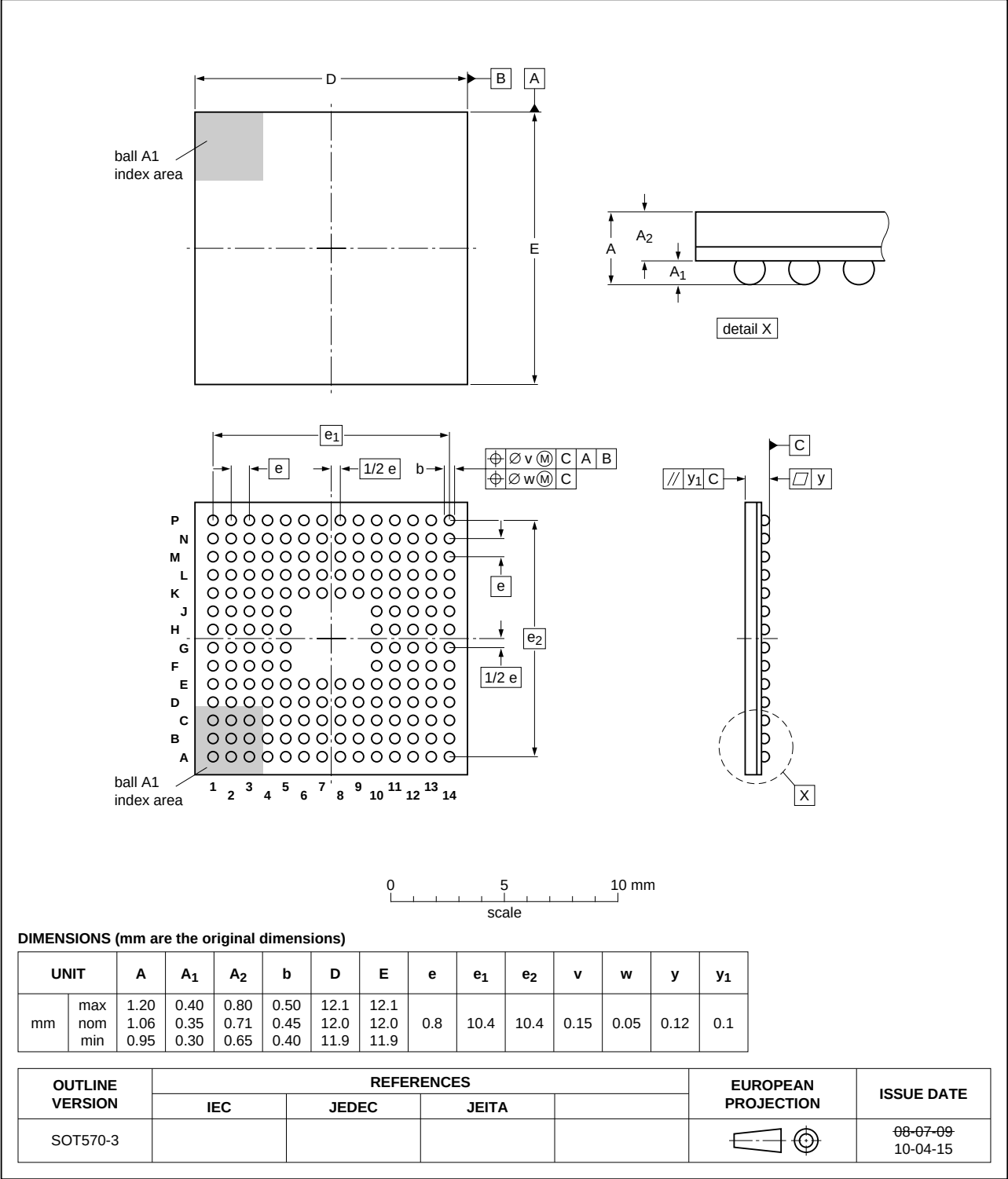
Fig 46. Package outline of the TFBGA180 package
