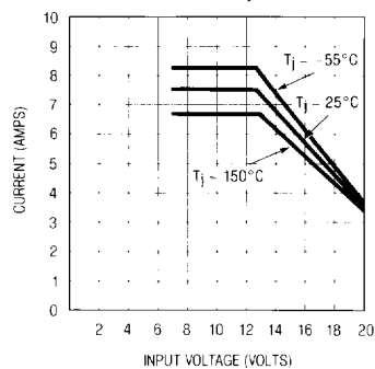
Peak Available Output Current
