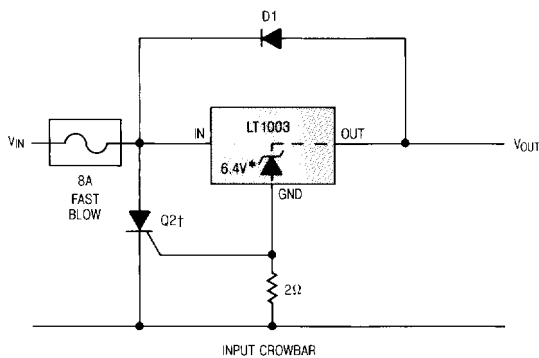
INPUT CROWBAR
