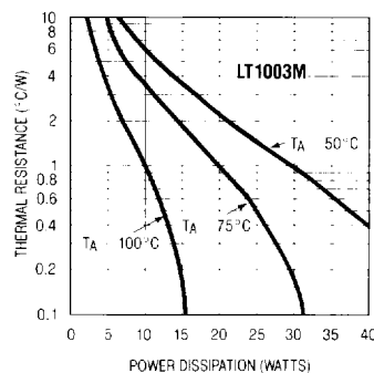
Suggested Heat Sink Thermal Resistance (LT1003M)
