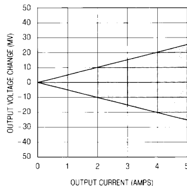
Load Regulation *
