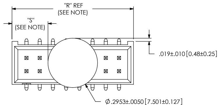
FIG 6 -K OPTION (POLYAMIDE FILM) LTMM-108-01-XX-D-SM-K SHOWN FOR SURFACE MOUNT OPTIONS ONLY (DIFFERENT AS SHOWN, OTHERWISE SAME AS FIG 3)
