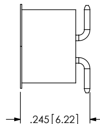
FIG 6 -K OPTION (POLYAMIDE FILM) LTMM-108-01-XX-D-SM-K SHOWN FOR SURFACE MOUNT OPTIONS ONLY (DIFFERENT AS SHOWN, OTHERWISE SAME AS FIG 3)
