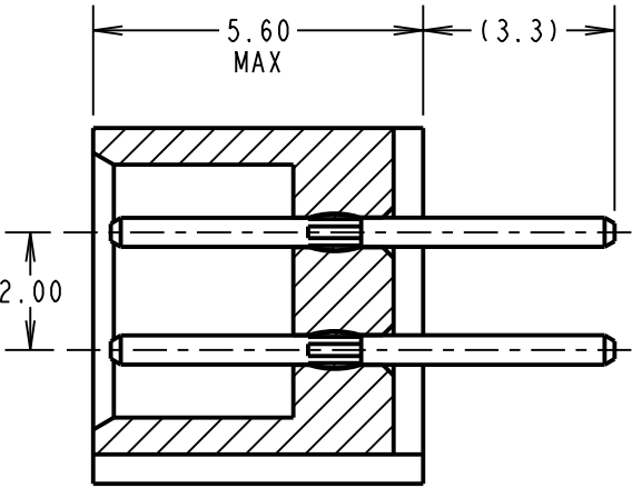
SECTION X-X
