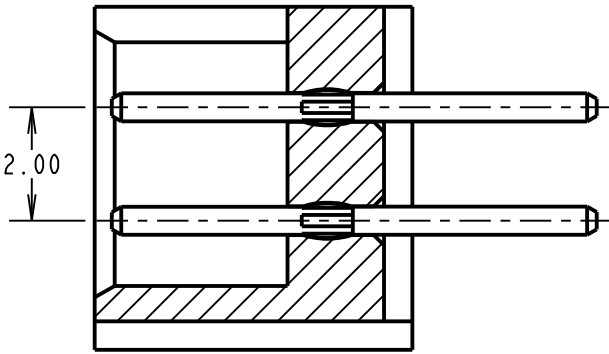
SECTION X-X
