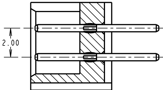
SECTION X-X
