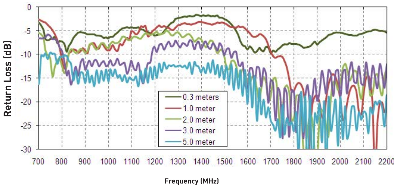
Figure 3. Return Loss of the MA104 antenna on 30*30cm metal plate
