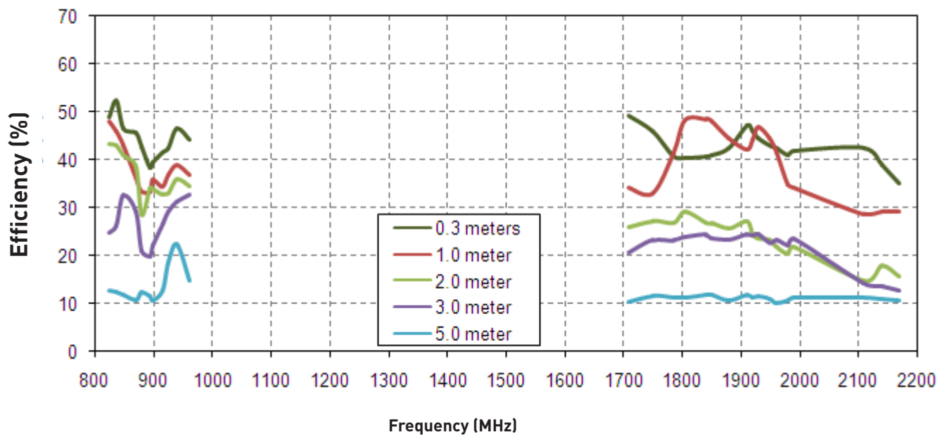
Figure 7. Efficiency of the MA104 antenna on 60*60cm metal plate.
