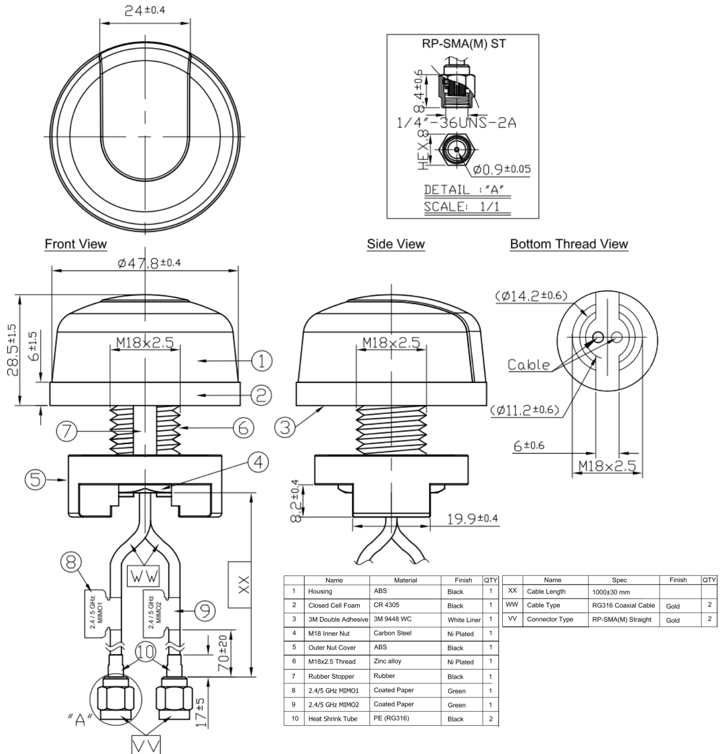
Figure 23. Antenna Drawing
