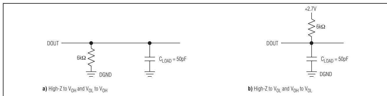
Figure 1. Load Circuits for DOOUT Enable Time
