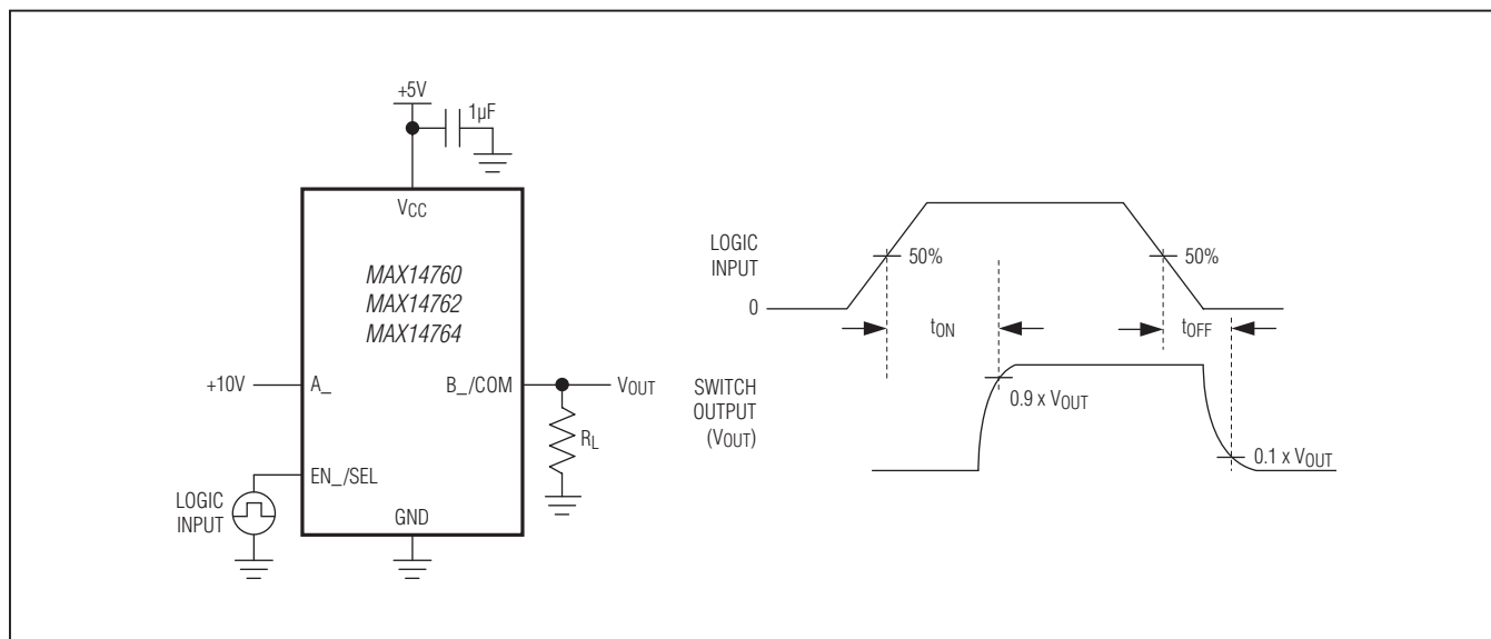
Figure 2. Switching Time
