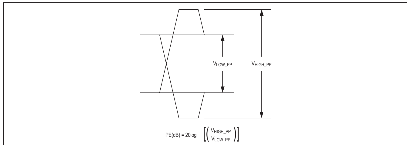
Figure 1. Output Preemphasis
