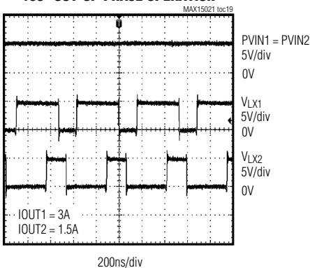
180° OUT-OF-PHASE OPERATION
