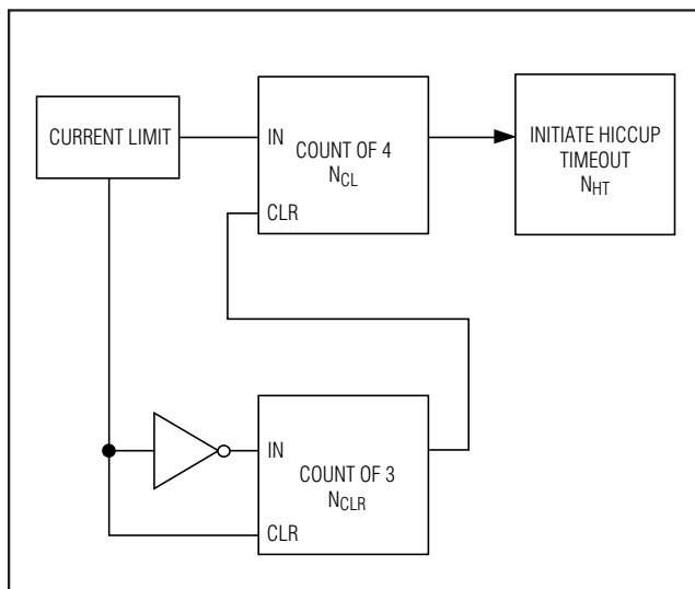
Figure 3. Hiccup-Mode Block Diagram
