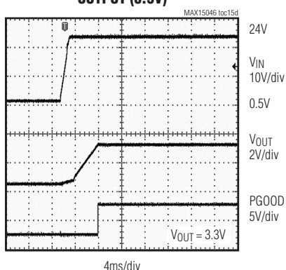
STARTUP WITH PREBIASED OUTPUT (0.5V)
