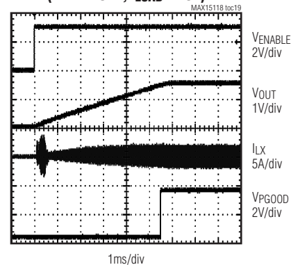
SOFT-START WAVEFORMS (PWM MODE, I_{LOAD} = 10A )
