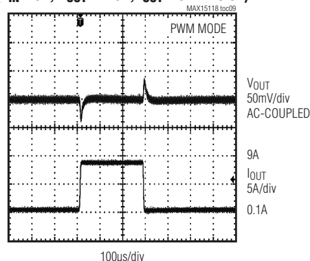
LOAD-TRANSIENT RESPONSE ( V_{IN} = 5V , V_{OUT} = 1.5V , I_{OUT} = 0.1A TO 9A )
