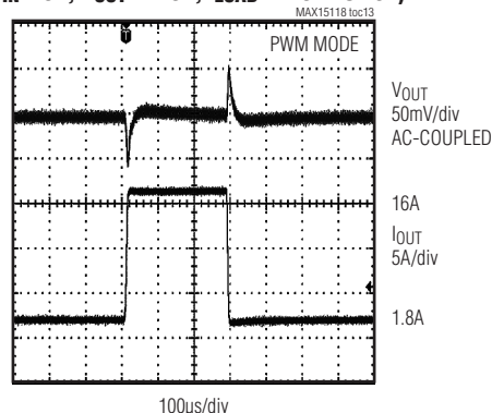
LOAD-TRANSIENT RESPONSE ( V_{IN} = 5V , V_{OUT} = 1.5V , I_{LOAD} = 1.8A TO 16A )
