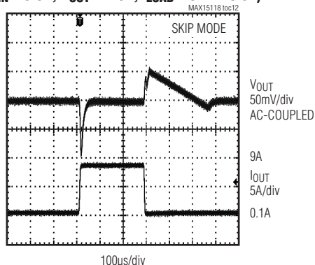
LOAD-TRANSIENT RESPONSE ( V_{IN} = 3.3V , V_{OUT} = 1.5V , I_{LOAD} = 0.1A TO 9A )
