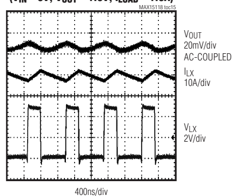
SWITCHING WAVEFORMS ( V_{IN} = 5V , V_{OUT} = 1.5V , I_{LOAD} = 1.8A )
