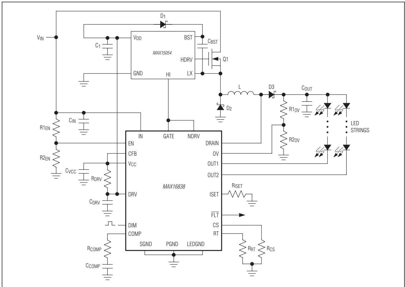
Figure 5. Boost-Buck Configuration
