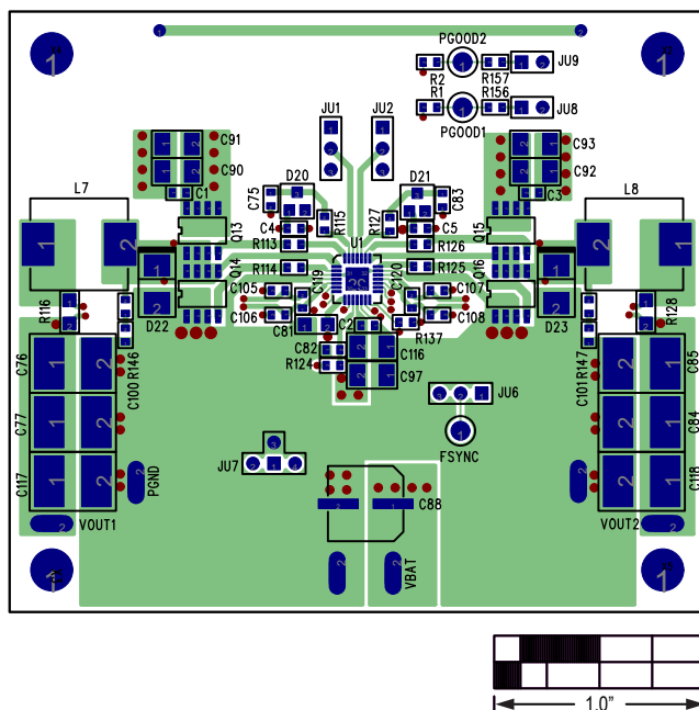
Figure 2. MAX16932 EV Kit Component Placement Guide—Component Side
