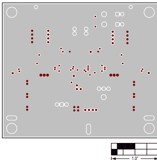
Figure 3. MAX16932 EV Kit PCB Layout—Component Side
