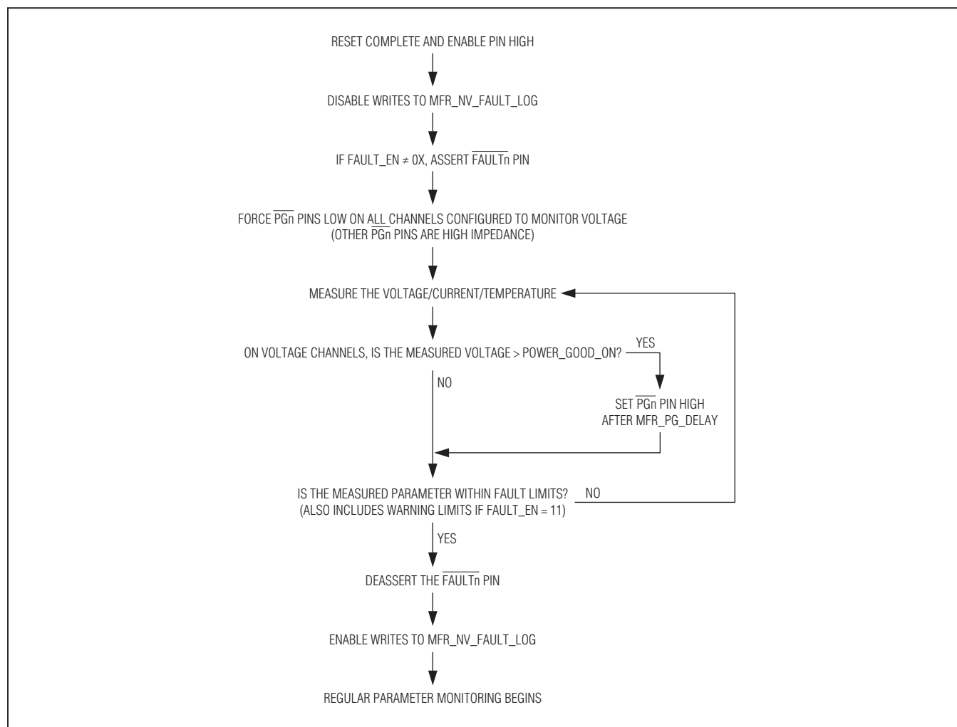
Figure 1. PGn and FAULTn Output After a Channel is Enabled
