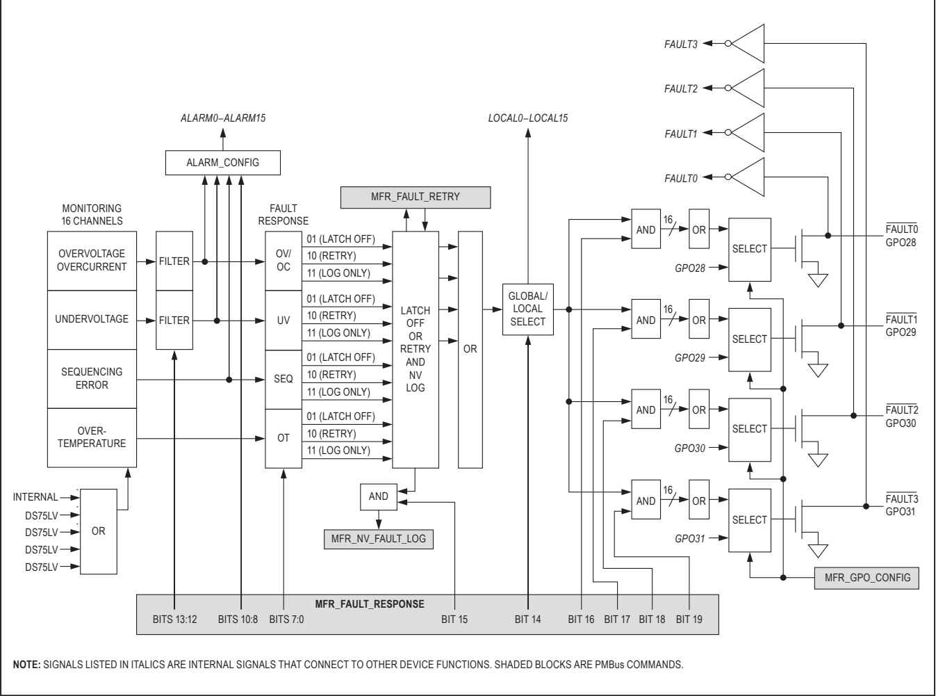
Figure 10. MFR_FAULT_RESPONSE Operation
