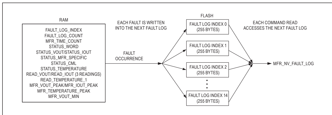
Figure 11. MFR_NV_FAULT_LOG
