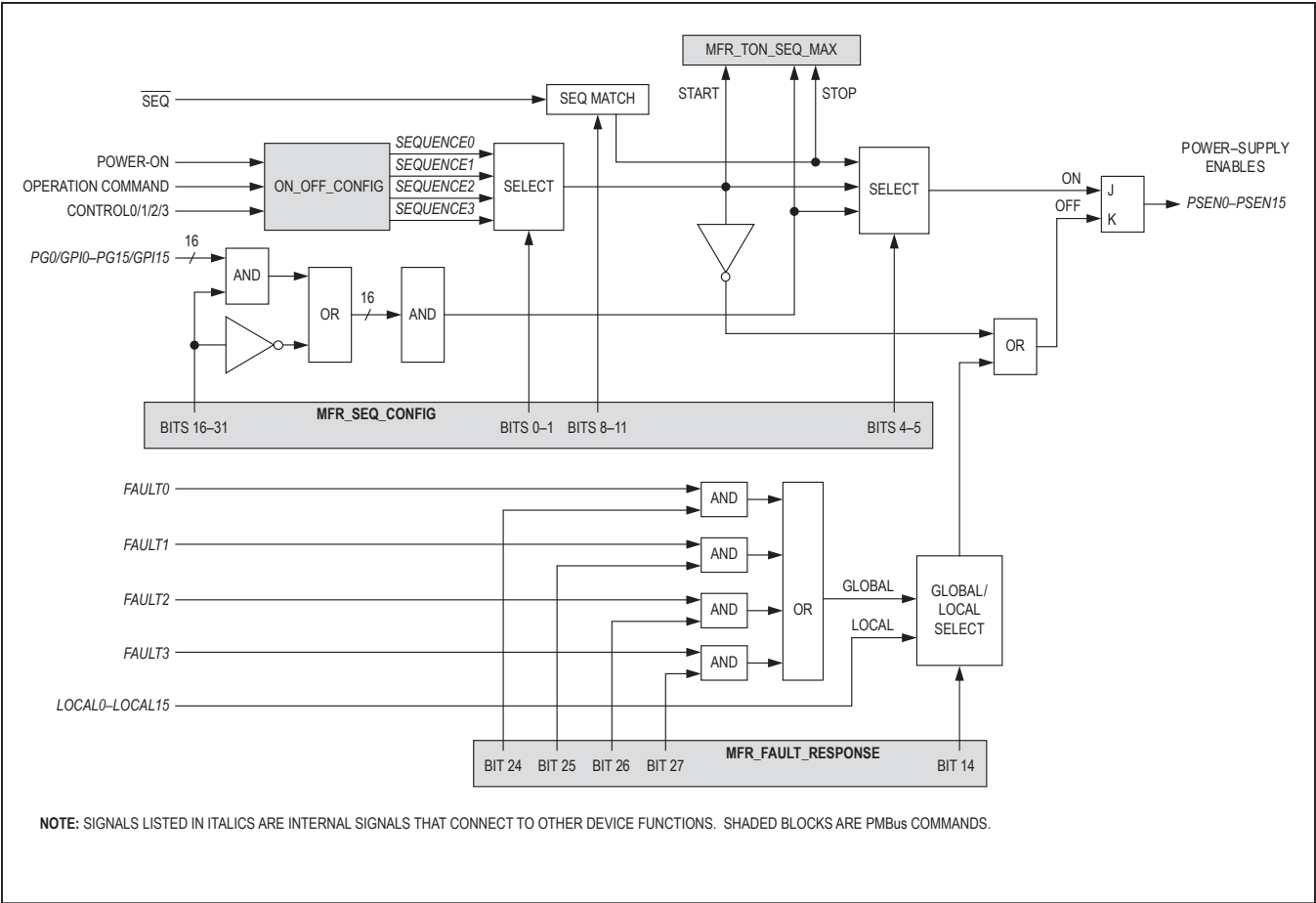
Figure 2. Sequence Control Logic
