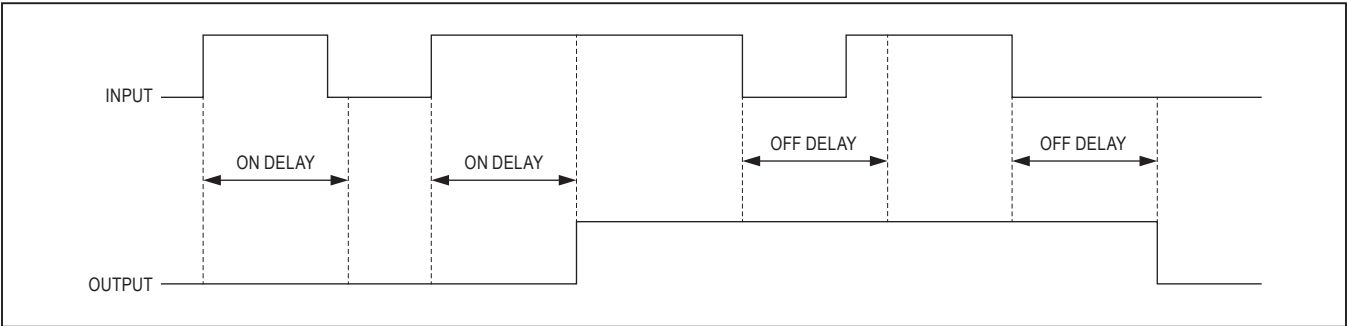
Figure 9. Input to Output Delay Action
