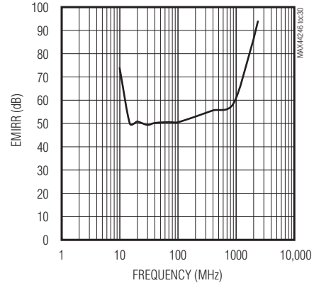
EMIRR vs. FREQUENCY ( V_{DD} = 3.3V )
