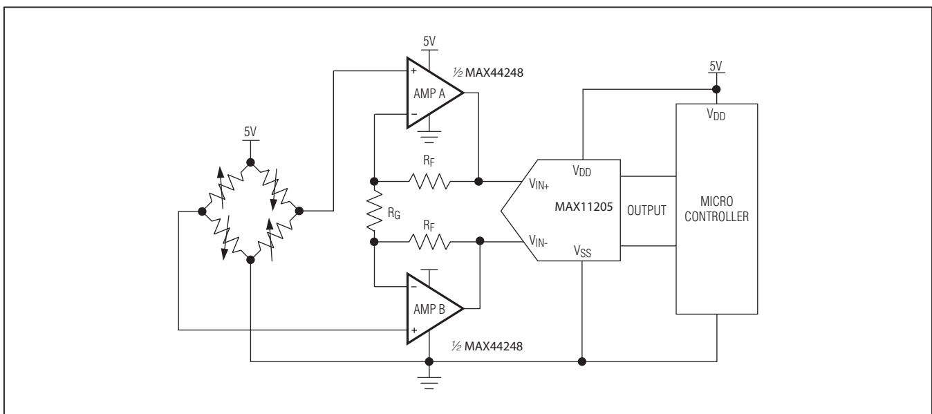
Figure 1. Weight Application
