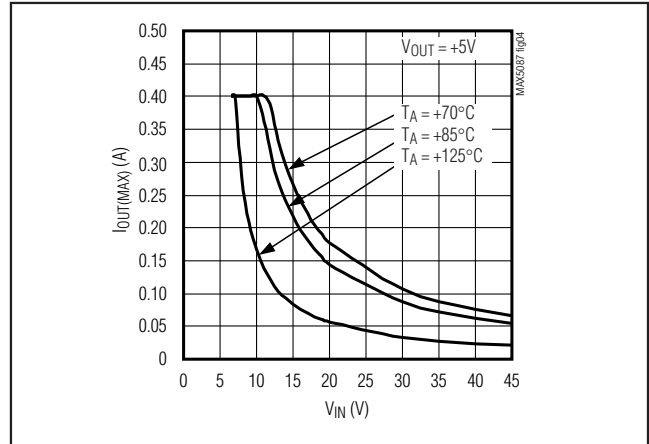
Figure 4. Maximum Output Current vs. Input Voltage (16-Pin TQFN)
