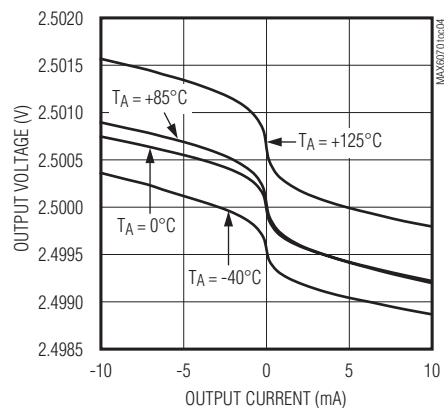
MAX6071_25 LOAD REGULATION
