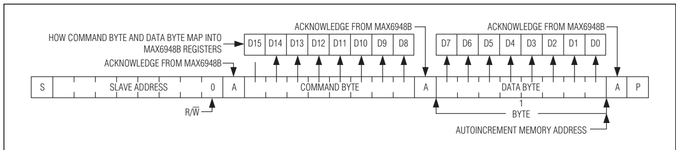
Figure 14. Command and Single Data Byte Received
