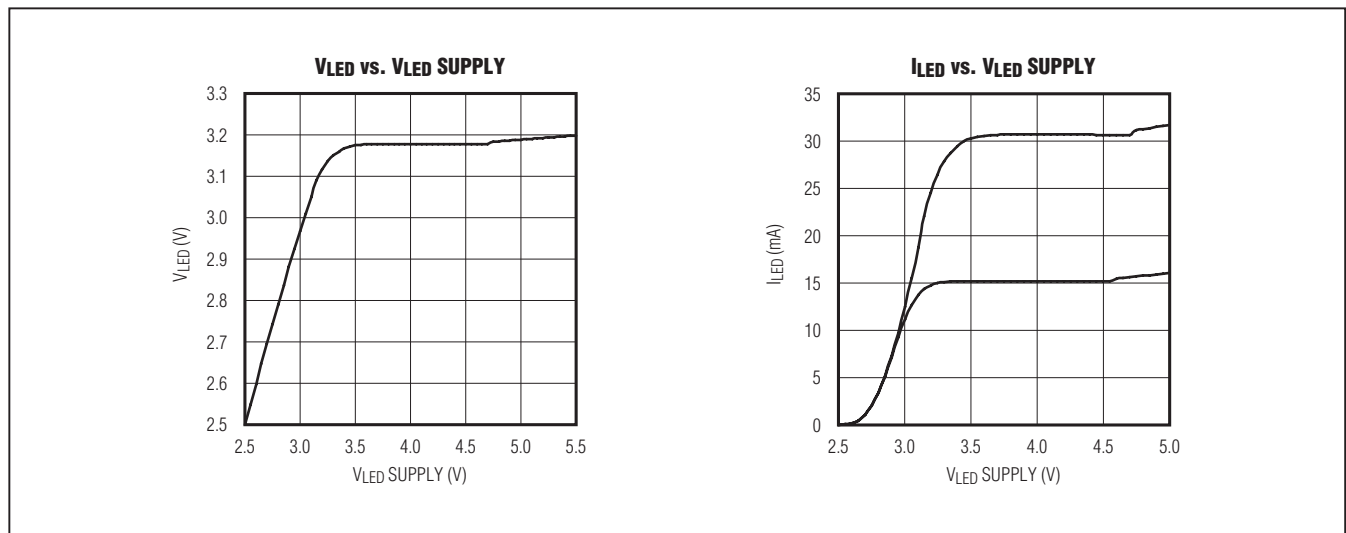
Figure 16. LED Brownout
