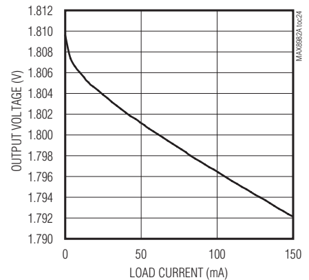
LD04 LOAD REGULATION
