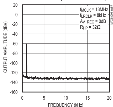
INBAND OUTPUT SPECTRUM, -60dBFS INPUT (DAC TO RECEIVER)
