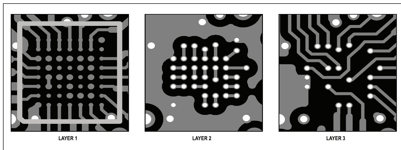
Figure 58. PCB Breakout Routing Example for WLP Package
