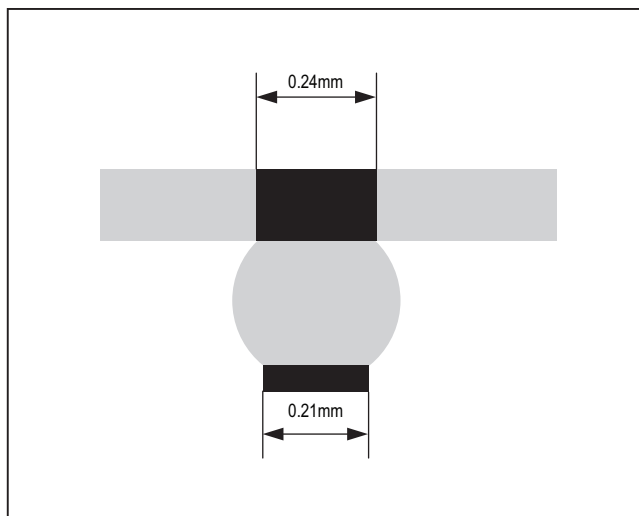
Figure 59. WLP Package Ball Dimensions
