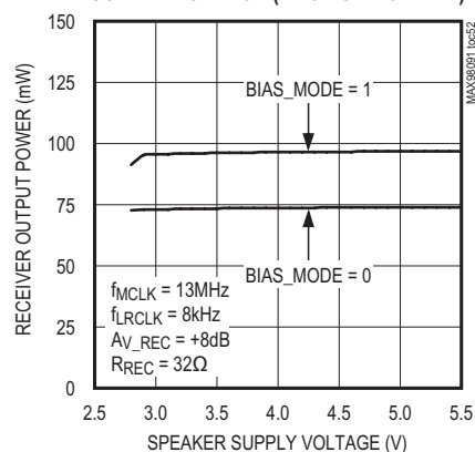
OUTPUT POWER vs. SPEAKER SUPPLY VOLTAGE (DAC TO RECEIVER)
