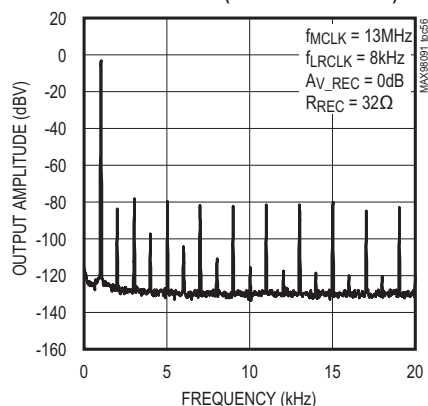
INBAND OUTPUT SPECTRUM, -3dBFS INPUT (DAC TO RECEIVER)
