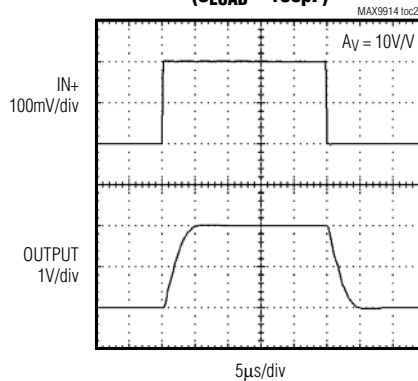
LARGE-SIGNAL PULSE RESPONSE ( C_{LOAD} = 100pF )
