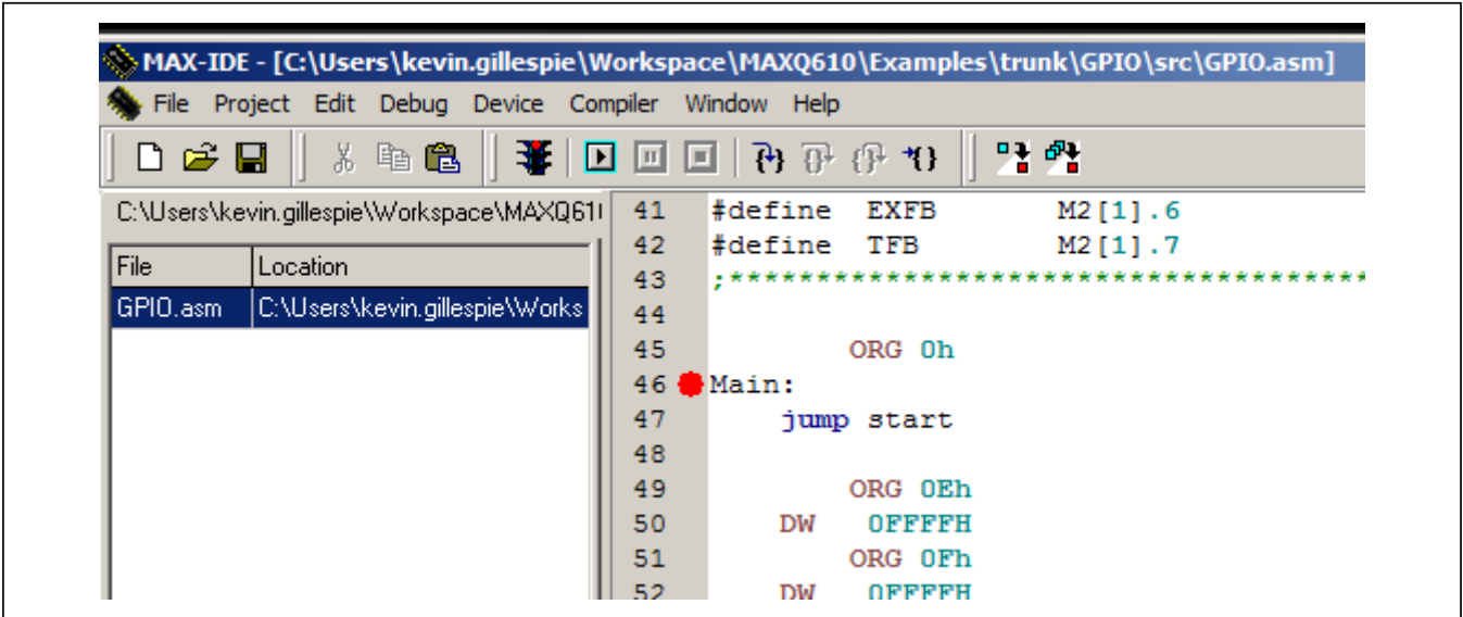
Figure 14. MAX-IDE Breakpoint
