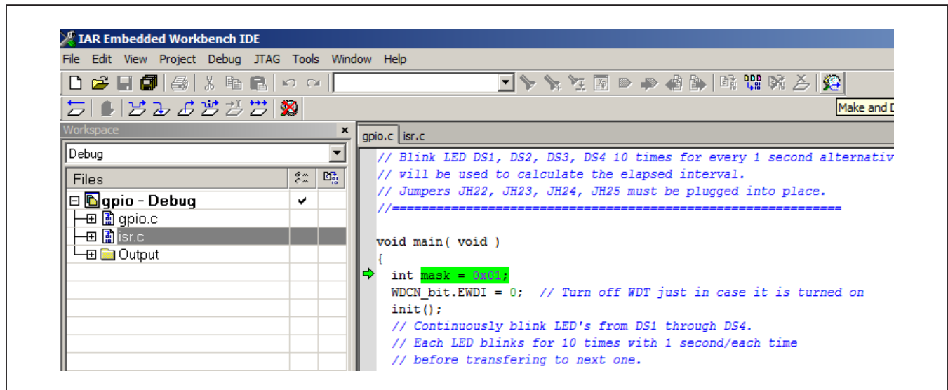
Figure 7. IAR Debugging
