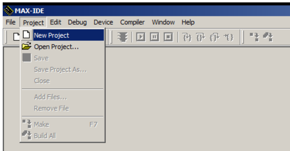
Figure 12. MAX-IDE Project
