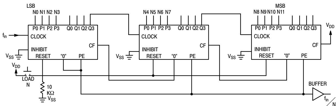
Figure 12. 3 Stages Cascaded
