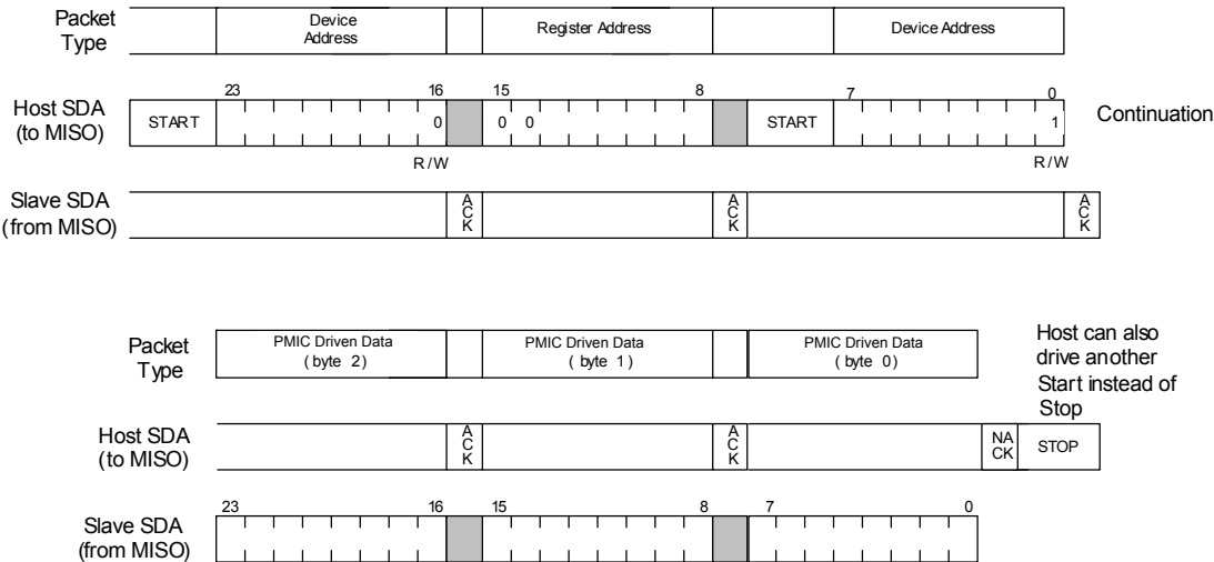
Figure 37. I 2 C 3-byte Read Example
