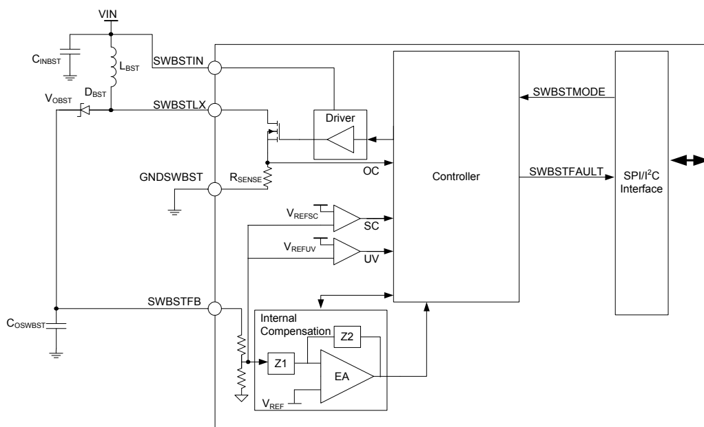
Figure 17. Boost Regulator Architecture
