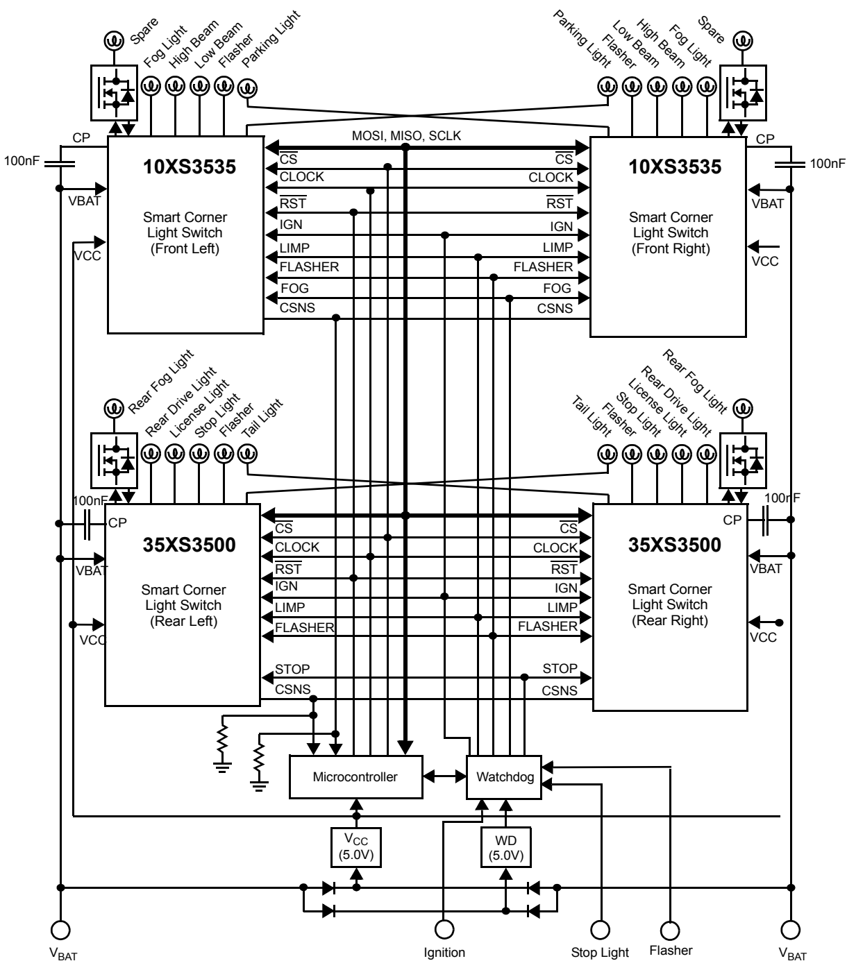
Figure 19. Typical Application
