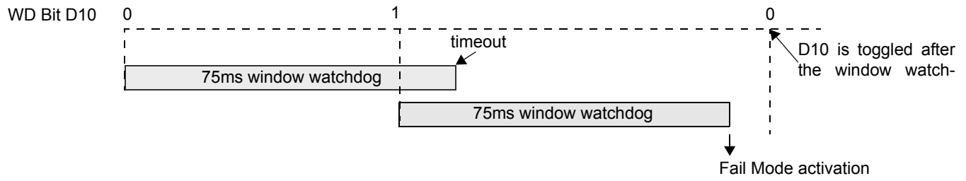
Figure 18. Watchdog Window
