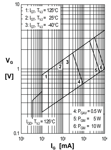
Fig. 5 Gate trigger charact.
