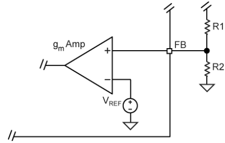
Figure 7. Voltage-Divider Configuration
