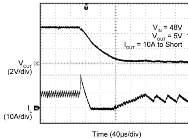
Short Circuit
