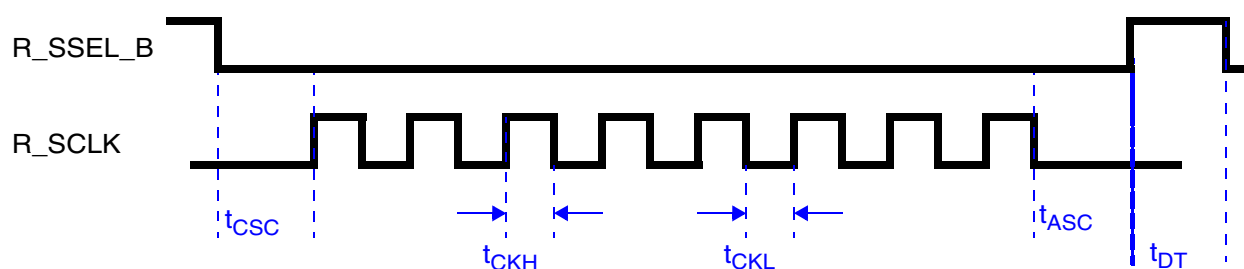
Figure 22. SPI timing: R_SSEL_B to R_SCLK
