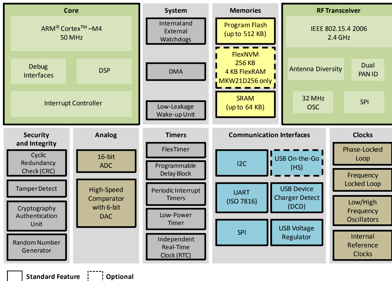
Figure 1. MKW2x simplified block diagram
