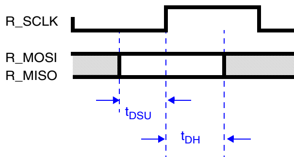
Figure 23. SPI timing: R_SCLK to R_MOSI and R_MISO
