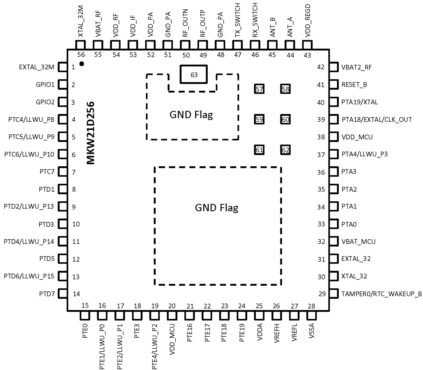
Figure 24. MKW21D256V Pin Assignment
