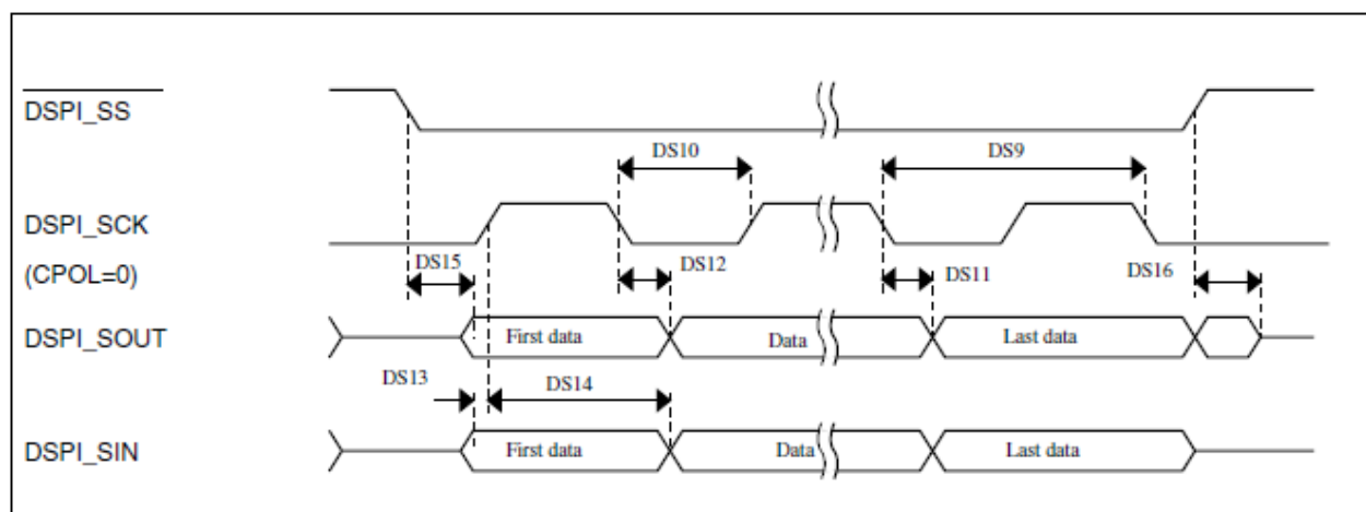
Figure 15. DSPI classic SPI timing — slave mode
