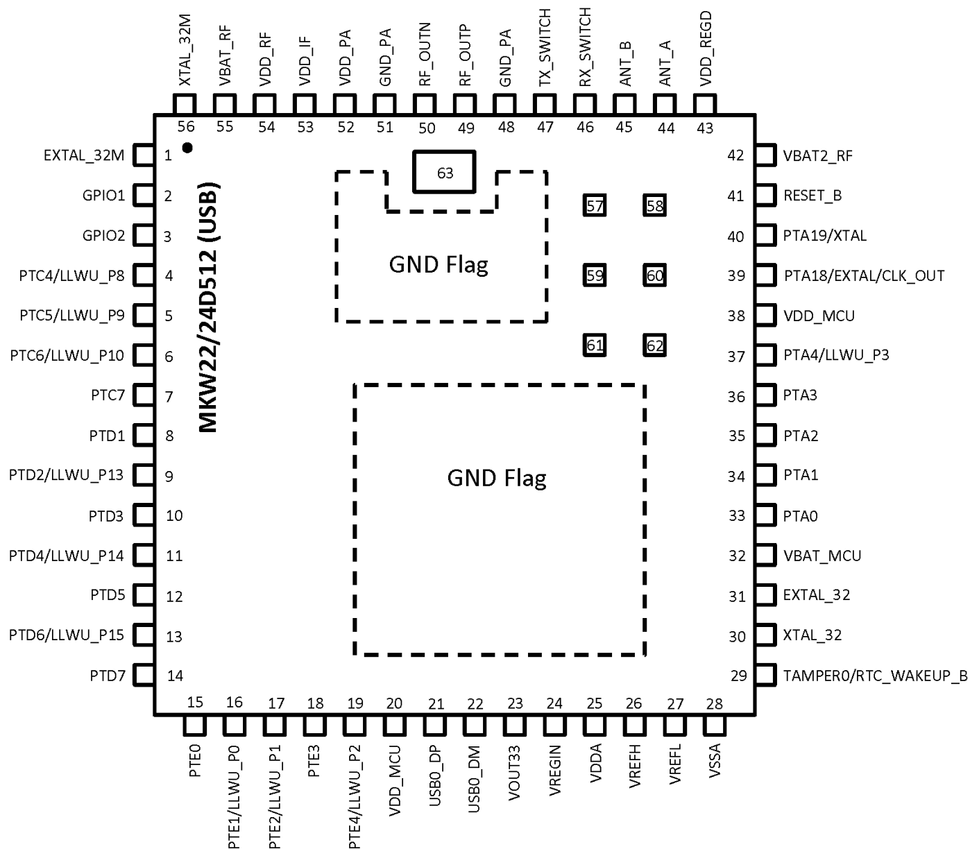
Figure 25. MKW22/24D512V (USB) Pin Assignment
