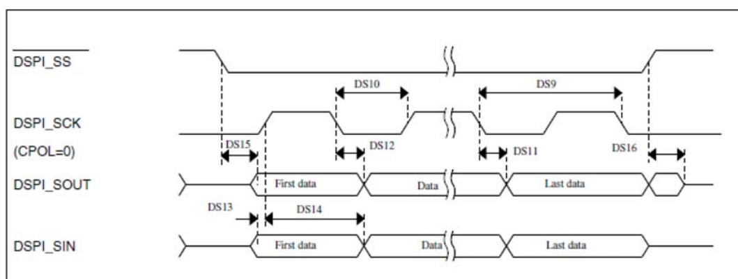
Figure 17. DSPI classic SPI timing — slave mode
