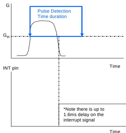
Figure 4. Single Pulse Detection
