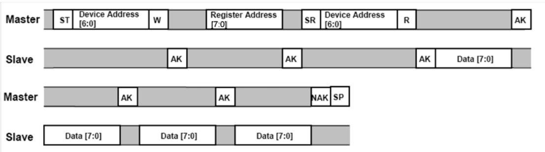
Figure 8. Multiple Bytes Read - The Master is reading multiple sequential registers from the MMA7456L
