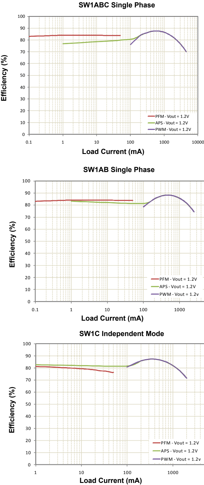
Figure 14. SW1AB and SW1C Efficiency Waveforms
