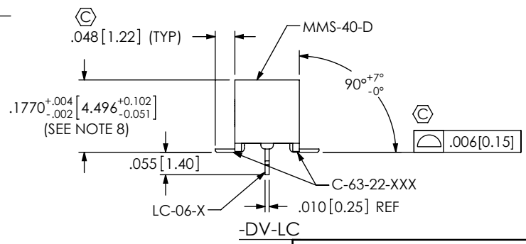
FIG 1 MMS-140-02-XXX-XV-LC SHOWN
