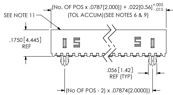
FIG 1 MMS-140-02-XXX-XV-LC SHOWN
