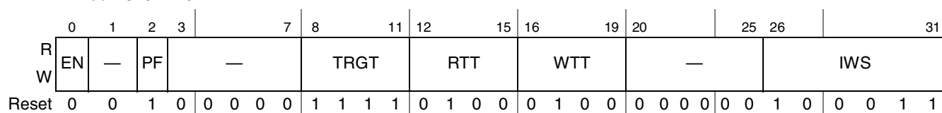
Figure 17-23. PCI Express Inbound Window Attributes Registers (PEXIWAR n )
