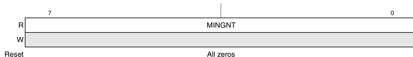
Figure 16-44. PCI Bus Minimum Grant Register (MIN_GNT)
