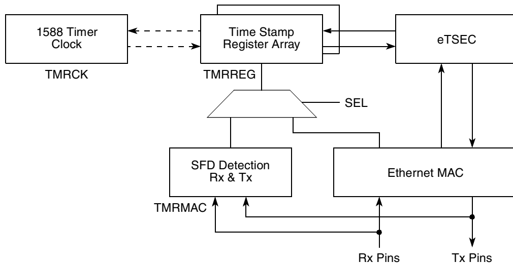
Figure 14-149. 1588 Timer Design Partition
