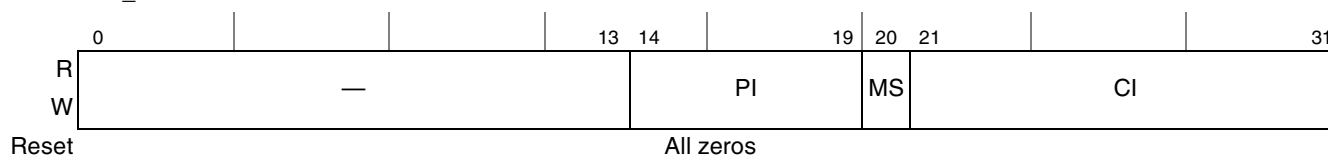
Figure 13-26. Flash Page Address Register, Large Page Device (OR \eta [PGS] = 1)
