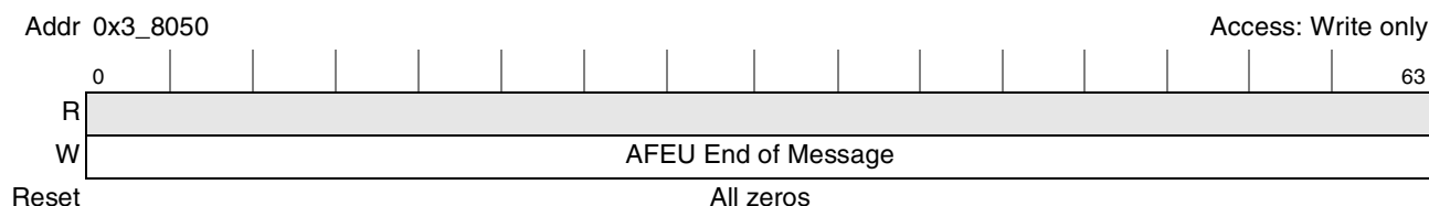
Figure 10-39. AFEU End of Message Register
