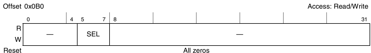
Figure 25-19. Trigger Out Source Register (TOSR)
