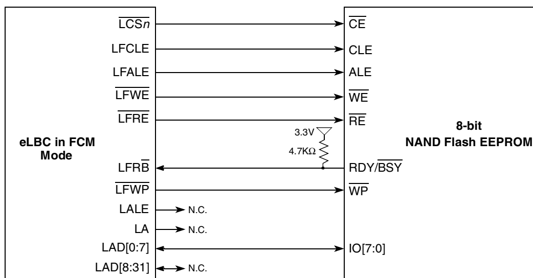
Figure 13-46. Local Bus to 8-Bit FCM Device Interface
