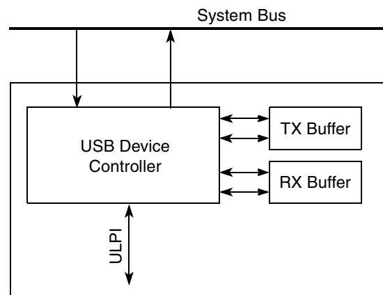
Figure 21-1. USB Interface Block Diagram
