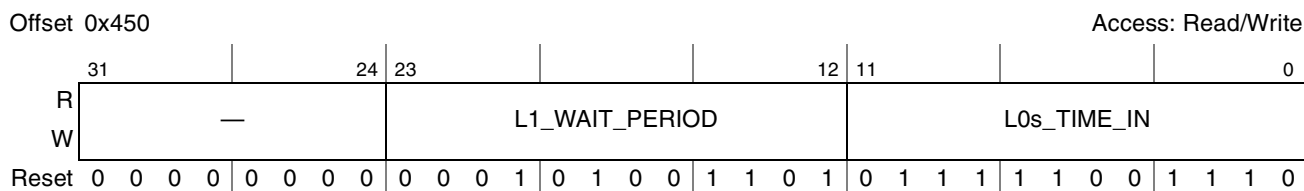
Figure 17-116. PCI Express Power Management Timer Register (PEX_PM_TIMER)
