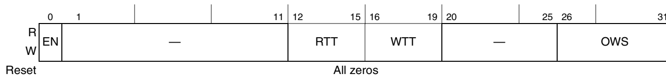
Figure 16-10. PCI Outbound Window 1–4 Attributes Registers (POWAR1–POWAR4)
