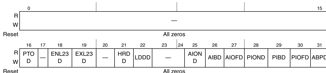
Figure 17-8. PCI Express PME and Message Disable Register (PEX_PME_MES_DISR)
