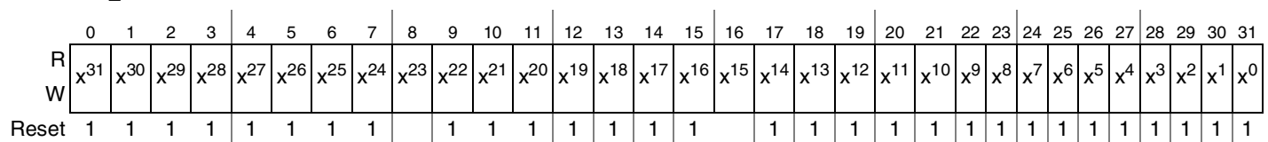
Figure 10-52. CRCU Context Register, Upper Half (Read in DOS Mode)
