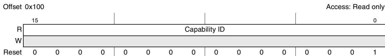
Figure 17-102. PCI Express Advanced Error Reporting Capability ID Register
