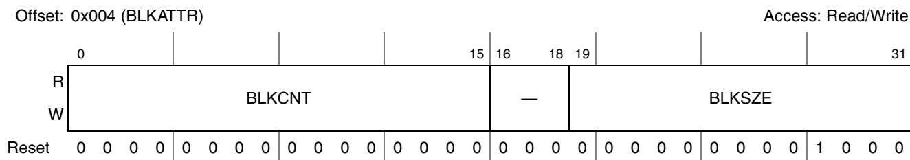
Figure 20-4. Block Attributes Register (BLKATTR)
