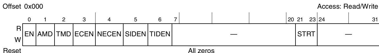
Figure 25-2. Watchpoint Monitor Control Register 0 (WMCRO)
