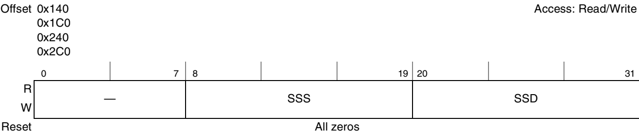
Figure 15-20. Source Stride Registers (SSR n )
