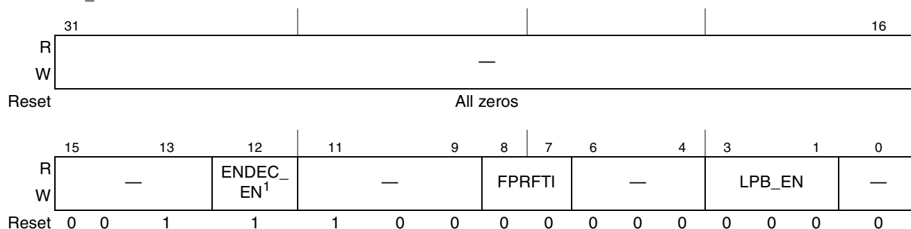
Figure 19-24. PHY Control Configuration Register1 (PhyCtrlCfg1)
