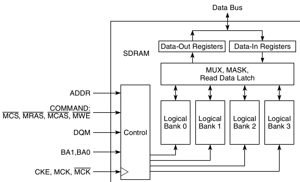
Figure 8-46. Typical Dual Data Rate SDRAM Internal Organization
