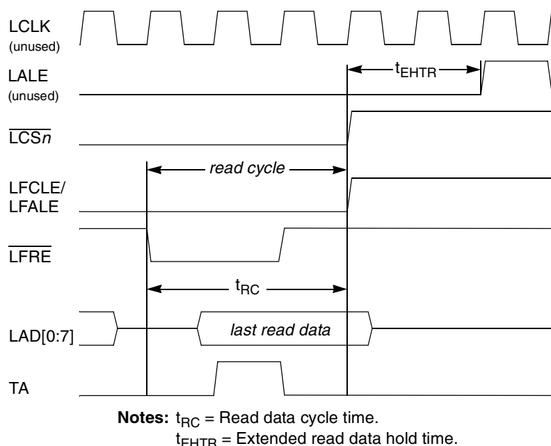
Figure 13-59. FCM Read Data Timing with Extended Hold Time (for TRLX = 0 , EHTR = 1 , RST = 1 , SCY = 1 )
