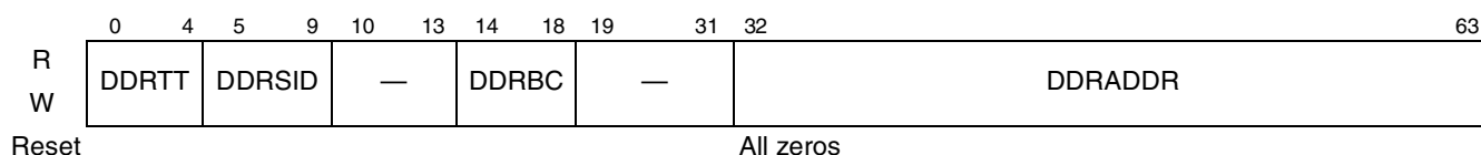
Figure 25-21. DDR Trace Buffer Entry
