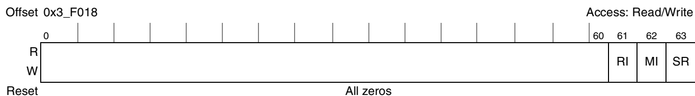
Figure 10-43. CRCU Reset Control Register
