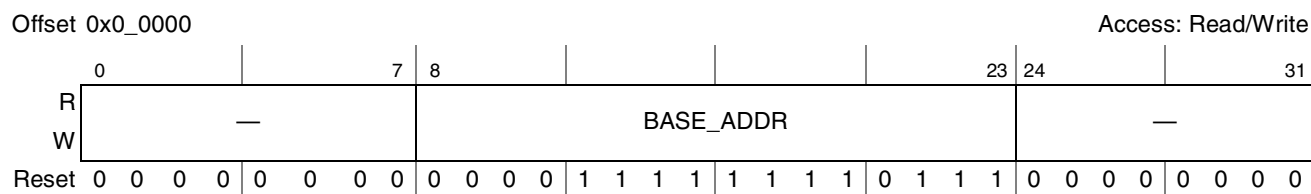
Figure 4-1. Configuration, Control, and Status Registers Base Address Register (CCSRBAR)
