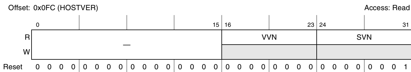
Figure 20-19. Host Controller Version Register (HOSTVER)
