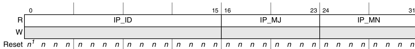
Figure 8-30. DDR IP Block Revision 1 (DDR_IP_REV1)
