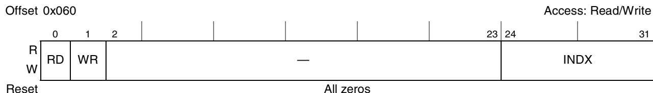
Figure 25-14. Trace Buffer Access Control Register (TBACR)
