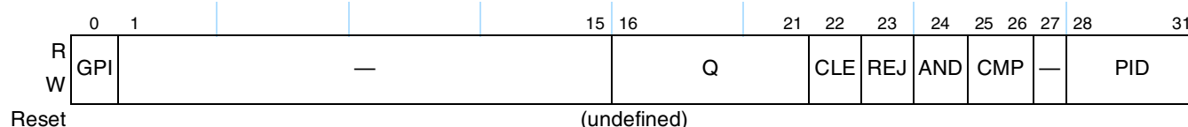
Figure 14-30. Receive Queue Filer Table Control Register Definition
