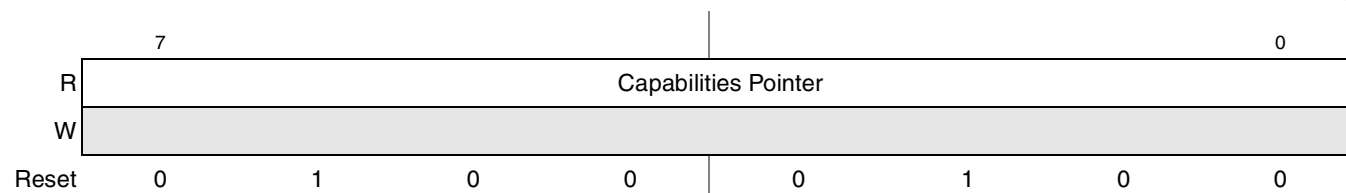
Figure 17-53. Capabilities Pointer Register
