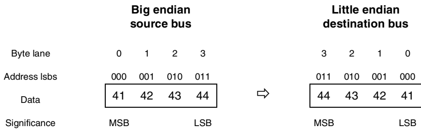
Figure 17-125. Address Invariant Byte Ordering—4 bytes Outbound
