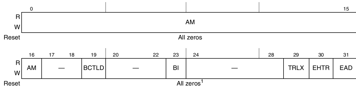
Figure 13-5. Option Registers (OR n ) in UPM Mode
