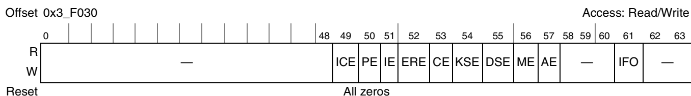
Figure 10-46. CRCU Interrupt Status Register
