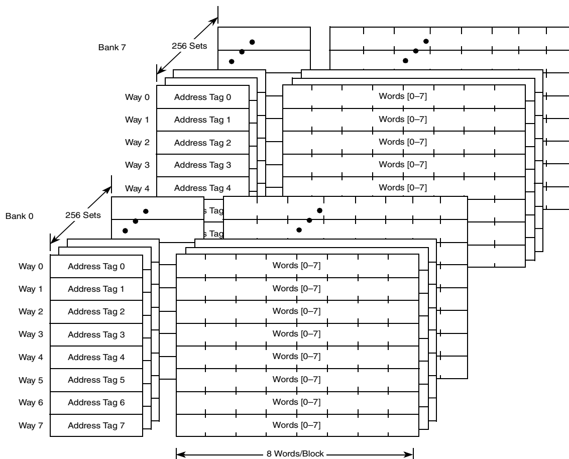
Figure 6-2. Cache Organization
