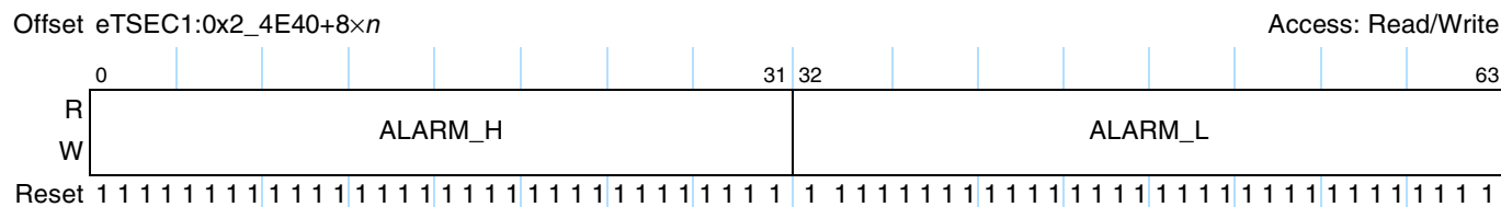
Figure 14-119. TMR_ALARM1-2_H/L Register Definition
