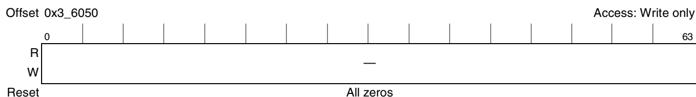
Figure 10-92. MDEU End of Message Register
