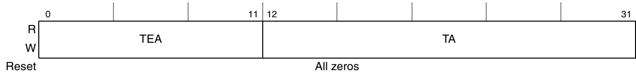
Figure 17-14. PCI Express Outbound Translation Address Registers (PEXOTAR n )
