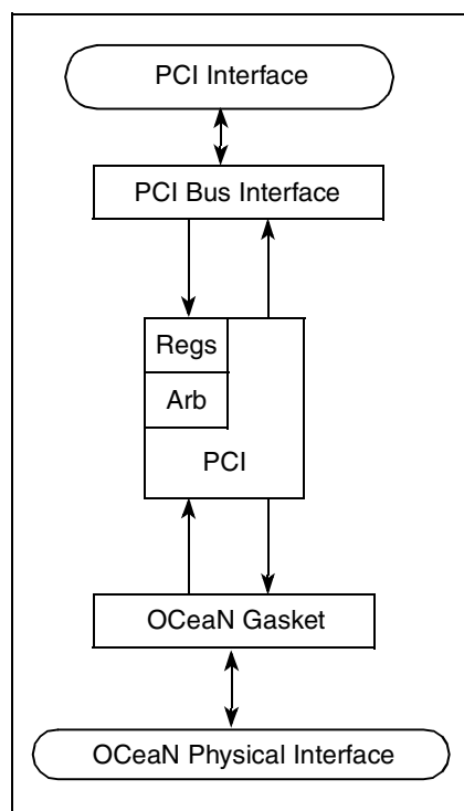
Figure 16-1. PCI Controller Block Diagram
