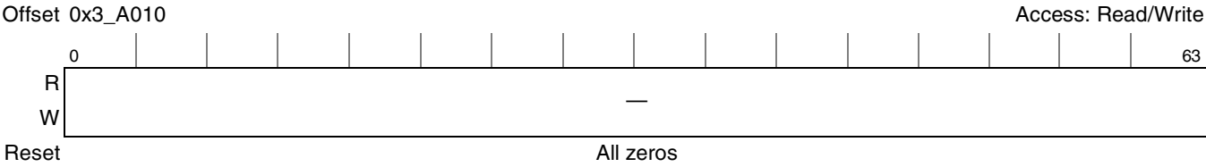
Figure 10-104. RNGU Data Size Register
