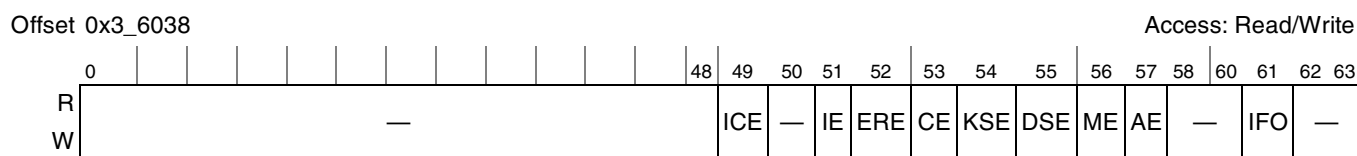
Figure 10-90. MDEU Interrupt Mask Register
