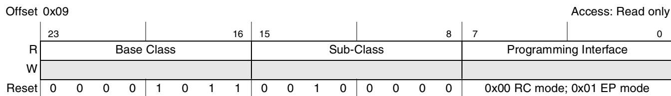
Figure 17-42. PCI Express Class Code Register
