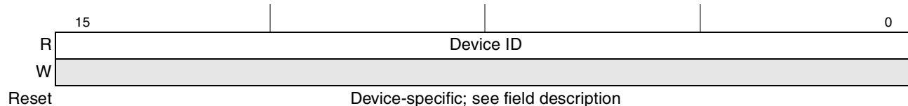
Figure 17-38. PCI Express Device ID Register
