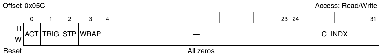
Figure 25-13. Trace Buffer Status Register (TBSR)
