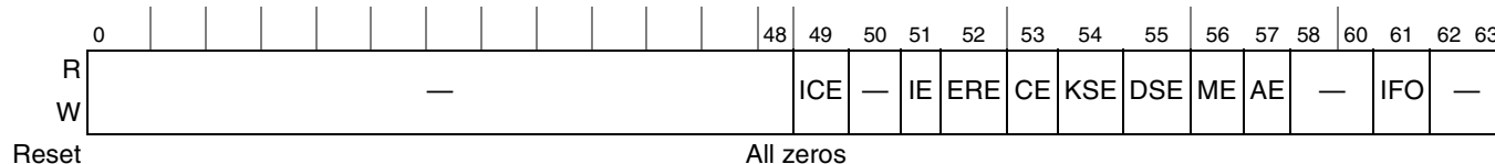
Figure 10-89. MDEU Interrupt Status Register
