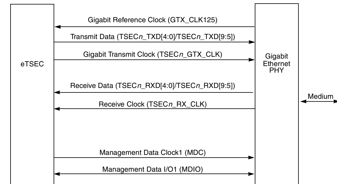
Figure 14-137. eTSEC-RTBI Connection
