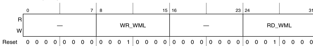
Figure 20-17. Watermark Level Register (WML)
