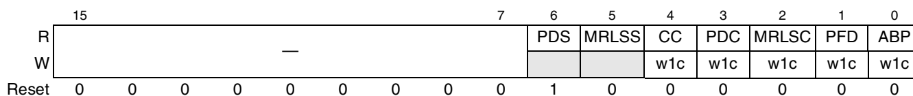
Figure 17-93. PCI Express Slot Status Register
