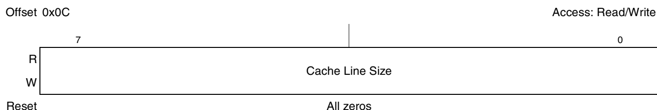
Figure 17-43. PCI Express Bus Cache Line Size Register
