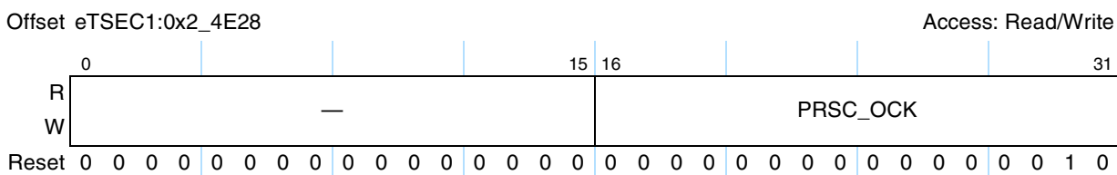
Figure 14-117. TMR_PRSC Register Definition
