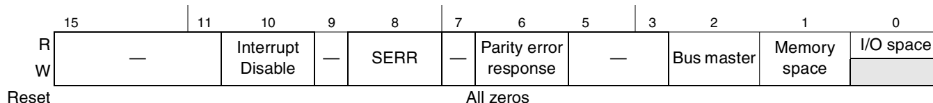
Figure 17-39. PCI Express Command Register
