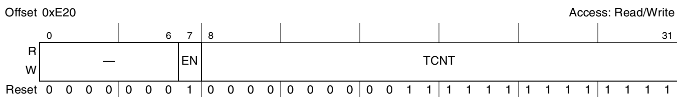
Figure 16-23. PCI Gasket Timer Register (GAS_TIMR)
