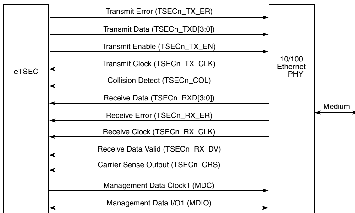
Figure 14-132. eTSEC-MII Connection
