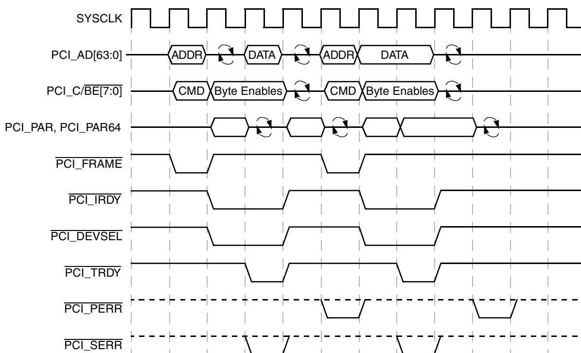
Figure 16-60. PCI Parity Operation
