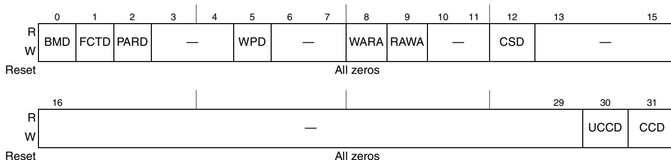
Figure 13-14. Transfer Error Check Disable Register (LTEDR)
