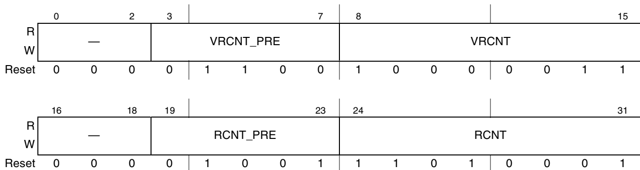
Figure 23-13. Power Management Reset Counters Configuration Register (PMRCCR)
