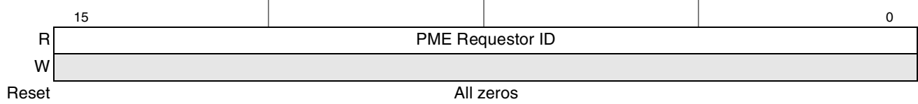
Figure 17-95. PCI Express Root Status Register
