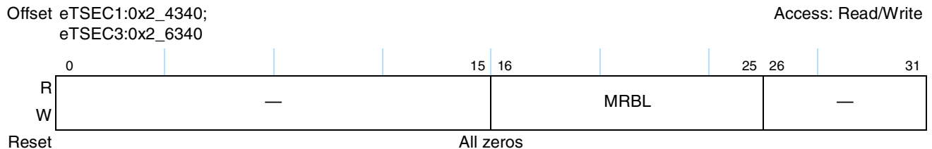
Figure 14-33. MRBLR Register Definition
