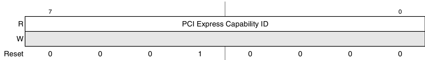
Figure 17-83. PCI Express Capability ID Register
