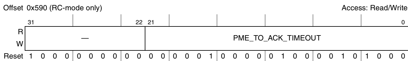
Figure 17-120. PCI Express PME To Ack Timeout Register (PEX PME TO ACK TOR)
