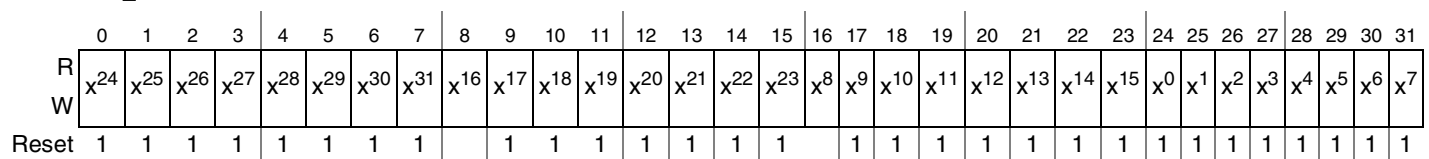
Figure 10-53. CRCU Context Register, Upper Half (Read in DOC Mode)
