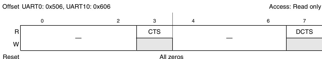
Figure 12-13. Modem Status Register (UMSR)
