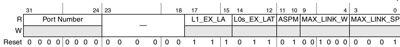
Figure 17-88. PCI Express Link Capabilities Register
