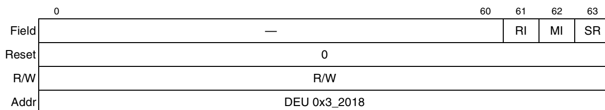
Figure 10-59. DEU Reset Control Register
