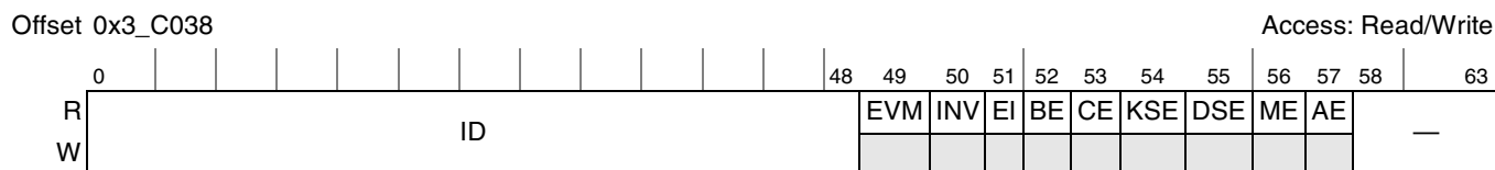
Figure 10-101. PKEU Interrupt Mask Register
