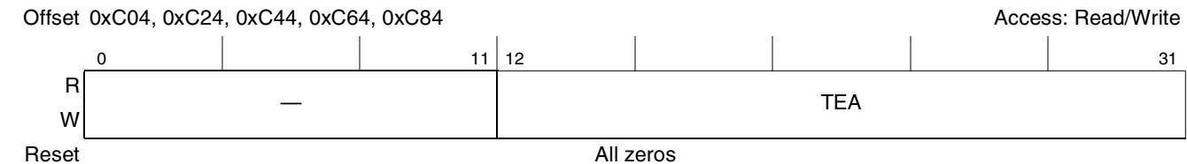
Figure 16-7. PCI Outbound Translation Extended Address Registers (POTEARN)
