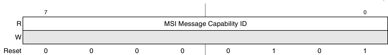
Figure 17-96. PCI Express Capability ID Register
