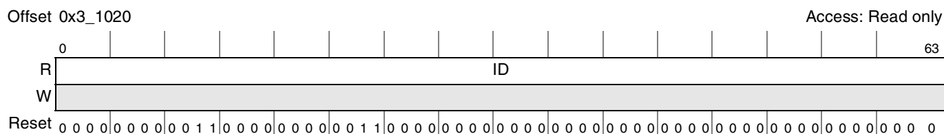
Figure 10-18. ID Register
