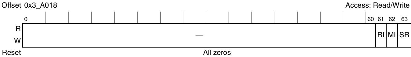
Figure 10-105. RNGU Reset Control Register
