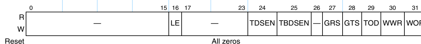
Figure 14-9. DMACTRL Register
