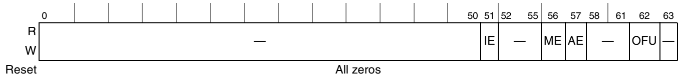
Figure 10-107. RNGU Interrupt Status Register
