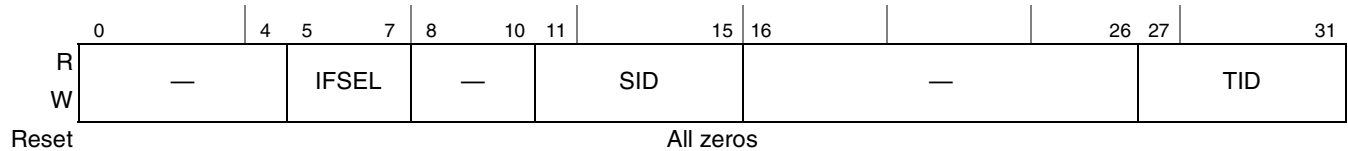
Figure 25-9. Trace Buffer Control Register 1 (TBCR1)
