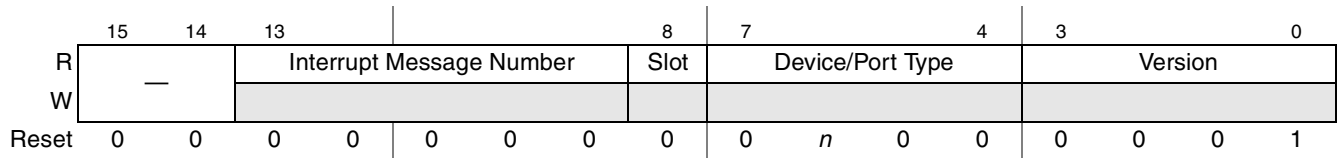
Figure 17-84. PCI Express Capabilities Register
