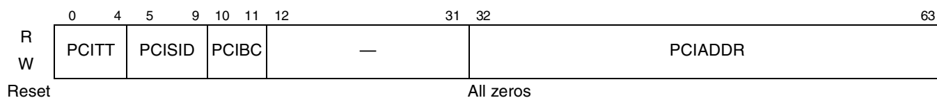
Figure 25-22. PCI Trace Buffer Entry
