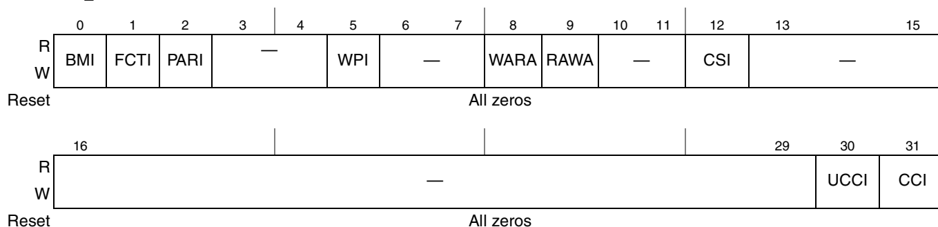
Figure 13-15. Transfer Error Interrupt Enable Register (LTEIR)
