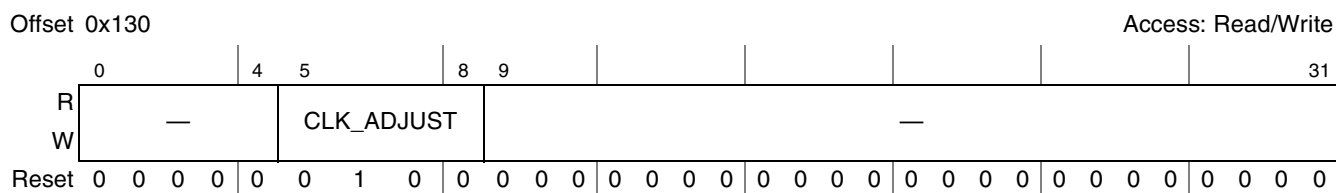
Figure 8-16. DDR SDRAM Clock Control Configuration Register (DDR_SDRAM_CLK_CNTL)
