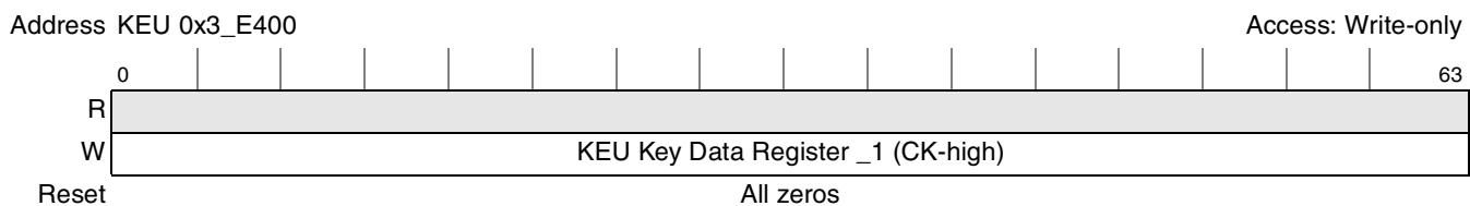
Figure 10-75. KEU Key Data Register_1 (CK-high)
