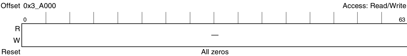
Figure 10-103. RNGU Mode Register
