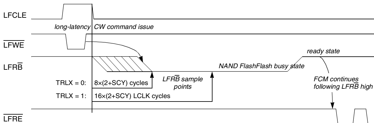
Figure 13-57. FCM Delay Prior to Sampling LFR\overline{B} State
