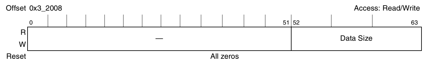
Figure 10-58. DEU Data Size Register
