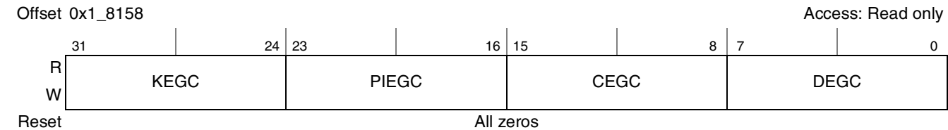
Figure 19-23. Link Layer Status Register1 (LinkStatus1)
