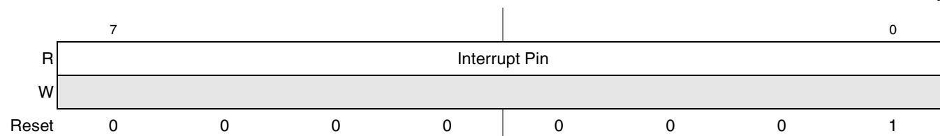
Figure 16-43. PCI Bus Interrupt Pin Register
