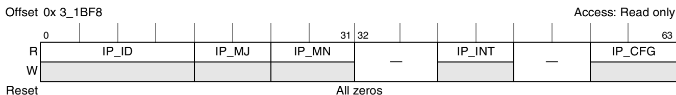
Figure 10-19. IP Block Revision Register
