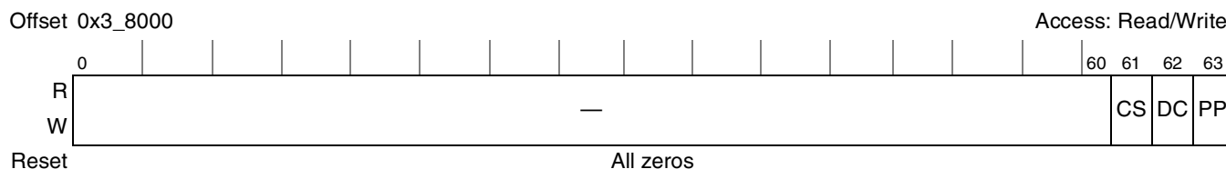
Figure 10-32. AFEU Mode Register
