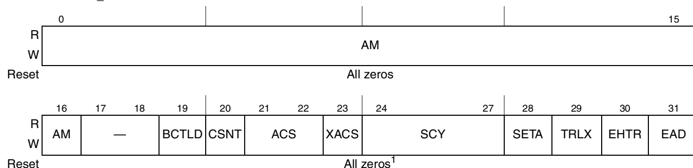
Figure 13-3. Option Registers (OR n ) in GPCM Mode
