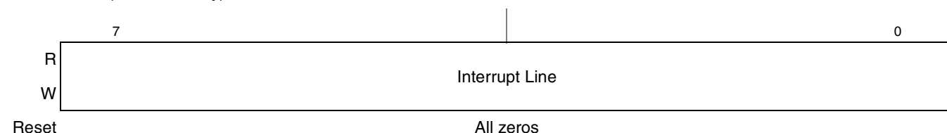
Figure 17-54. PCI Express Interrupt Line Register
