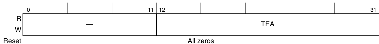
Figure 17-15. PCI Express Outbound Translation Extended Address Registers (PEXOTEAR n )
