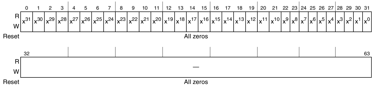
Figure 10-50. CRCU Context Register (Write)
