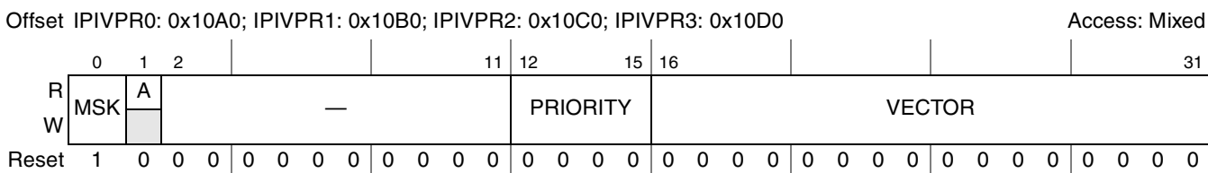
Figure 9-9. Interprocessor Interrupt Vector/Priority Register (IPIVPR n )
