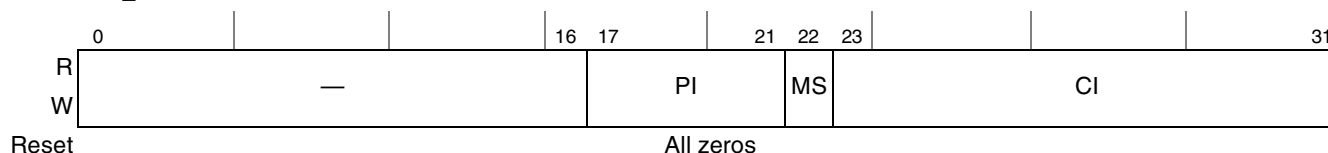
Figure 13-25. Flash Page Address Register, Small Page Device (OR \eta [PGS] = 0)
