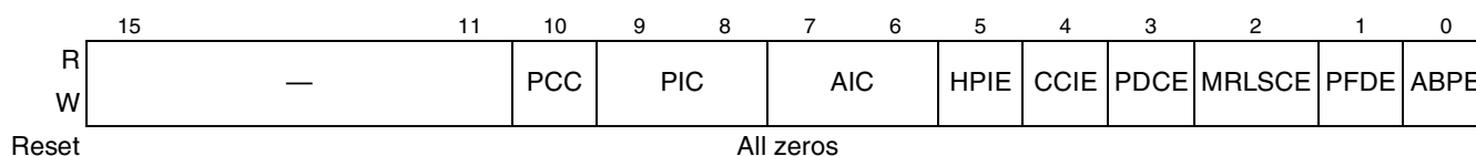
Figure 17-92. PCI Express Slot Control Register
