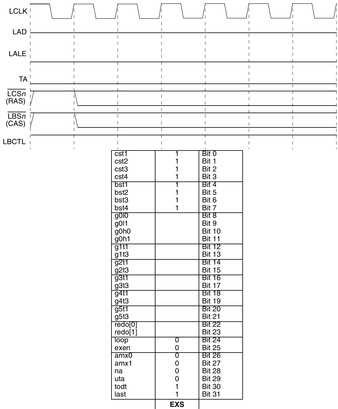
Figure 13-80. Exception Cycle
