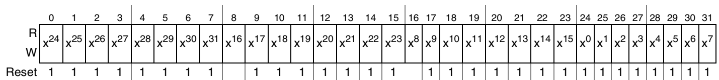
Figure 10-51. CRCU Context Register, Upper Half (Read in Default Mode)
