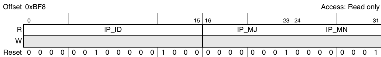
Figure 17-11. IP Block Revision Register 1
