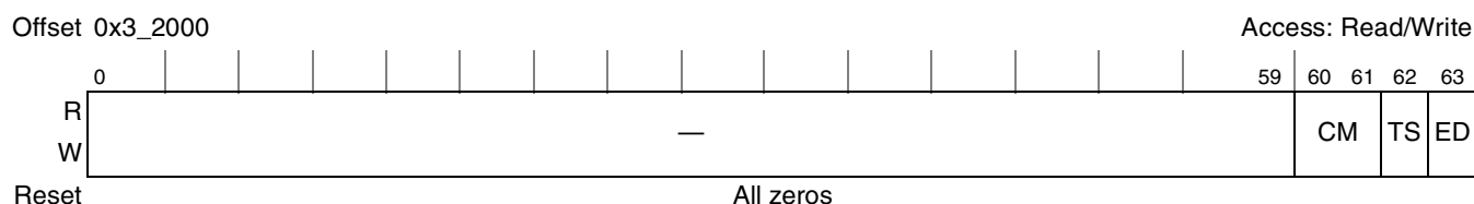
Figure 10-56. DEU Mode Register
