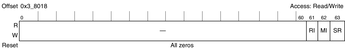
Figure 10-35. AFEU Reset Control Register
