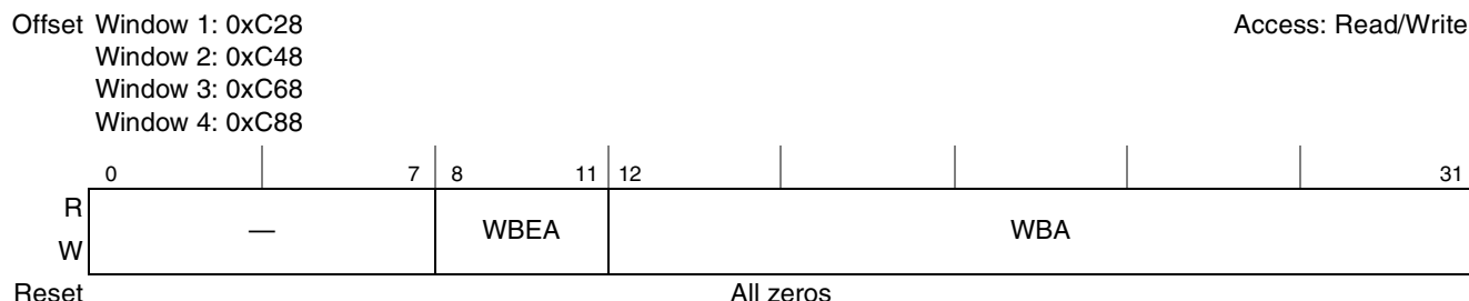
Figure 17-16. PCI Express Outbound Window Base Address Registers (PEXOWBAR n )
