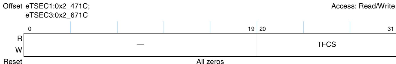
Figure 14-93. Transmit FCS Error Counter Register Definition
