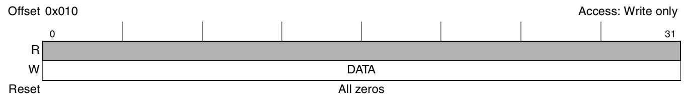
Figure 18-7. eSPI Transmit Data Register (SPITF)
