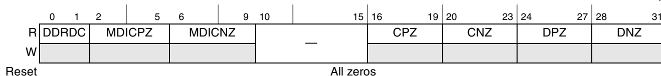
Figure 8-26. DDR Debug Status Register 1 (DDRDSR_1)
