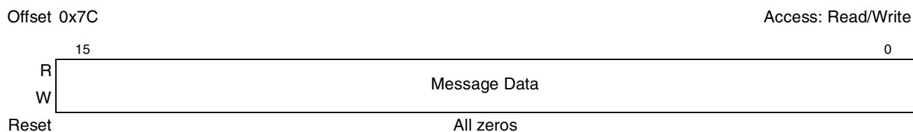
Figure 17-100. PCI Express MSI Message Data Register
