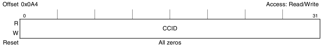
Figure 25-18. Current Context ID Register (CCIDR)
