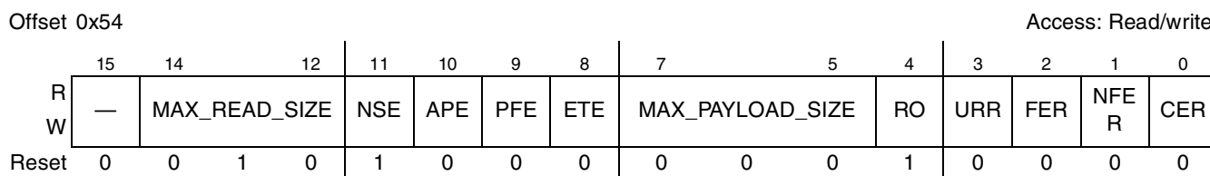
Figure 17-86. PCI Express Device Control Register
