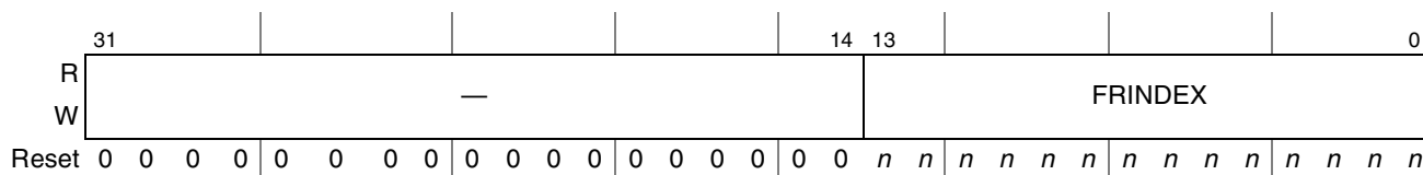
Figure 21-11. USB Frame Index (FRINDEX)
