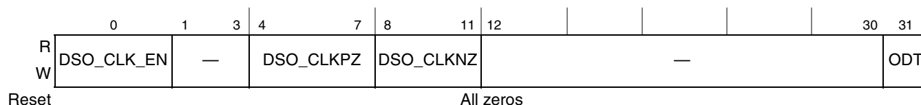
Figure 8-29. DDR Control Driver Register 2 (DDRCDR_2)
