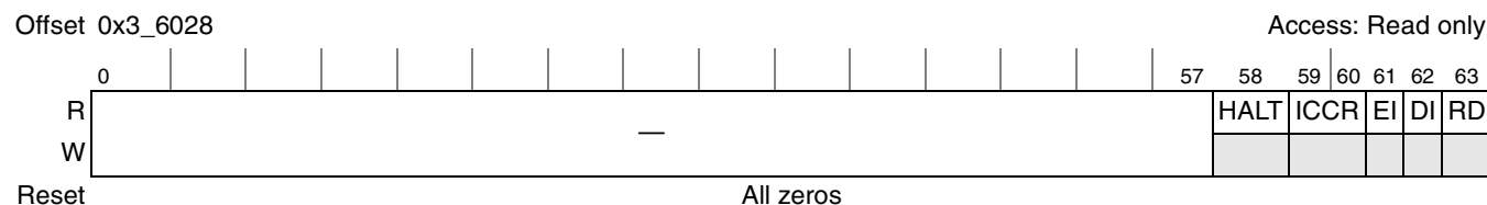
Figure 10-88. MDEU Status Register
