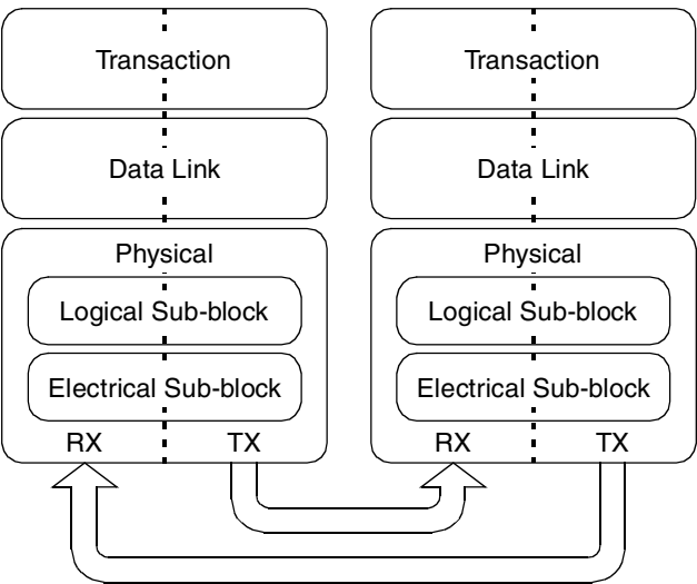
Figure 17-123. PCI Express High-Level Layering
