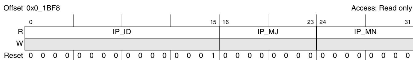
Figure 7-4. ECM IP Block Revision Register 1 (EIPBRR1)
