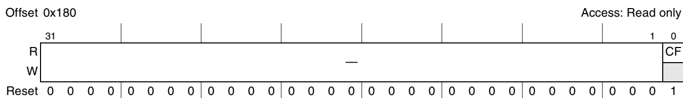
Figure 21-19. Configure Flag Register (CONFIGFLAG)
