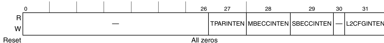
Figure 6-21. L2 Error Interrupt Enable Register (L2ERRINTEN)
