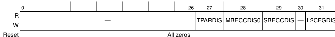
Figure 6-20. L2 Error Disable Register (L2ERRDIS)
