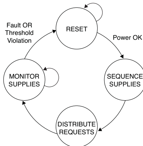
Figure 3. Power Manager II POWR1014A Embedded Logic
