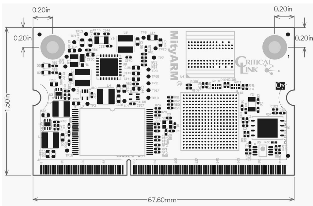
Figure 2 MityARM-3359 Mechanical Outline
