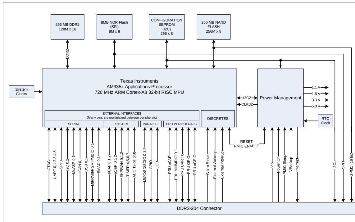
Figure 1 MityARM-3359 Block Diagram
