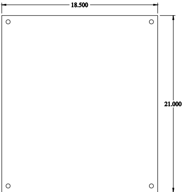
INNER PANEL
