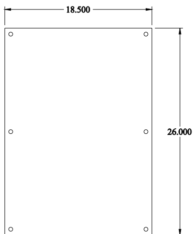
INNER PANEL
