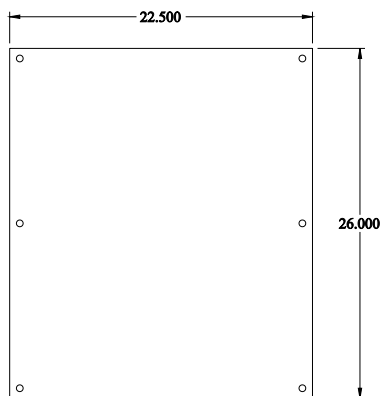
INNER PANEL
