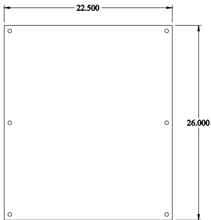
INNER PANEL
