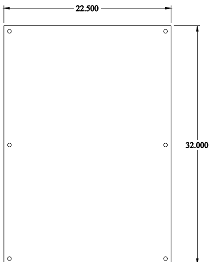
INNER PANEL
