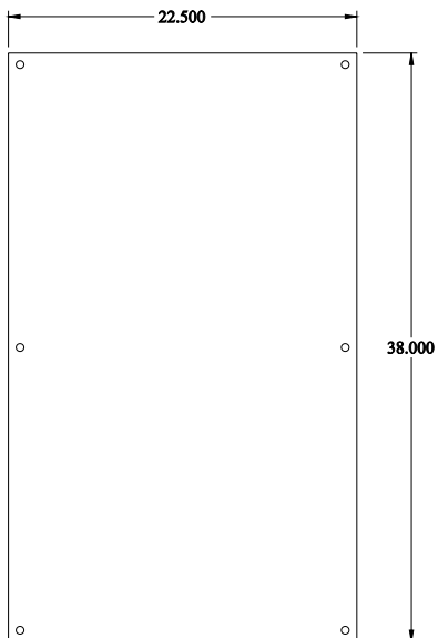
INNER PANEL
