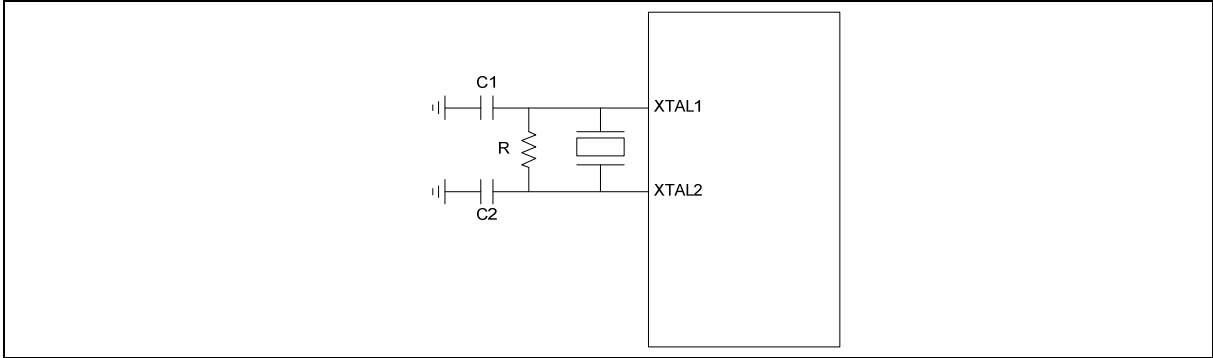
Figure 31-1 Typical Crystal Application Circuit
