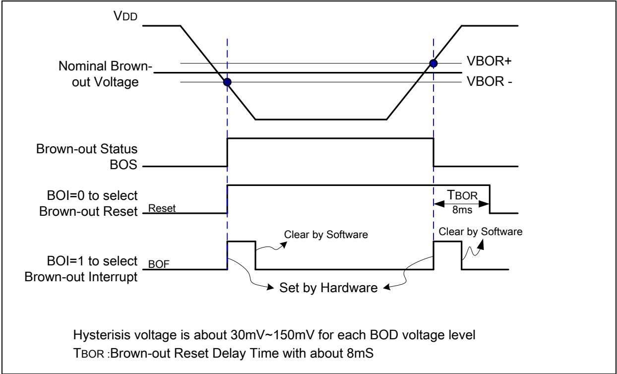
Figure 24-2: Brown-out Voltage Detection
