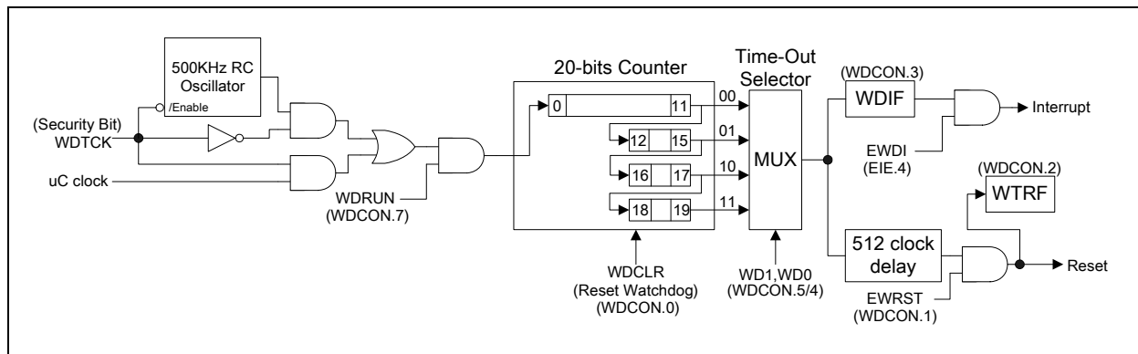
Figure 14-1 Watchdog Timer
