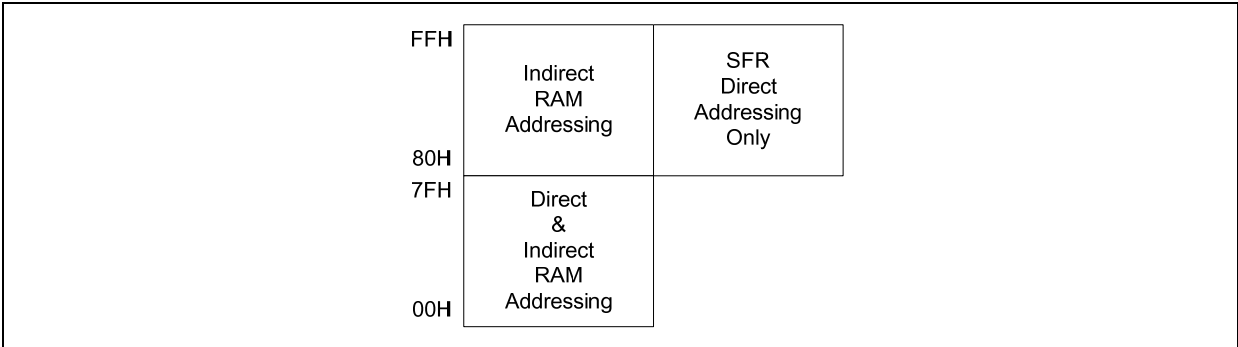
Figure 6-2 N79E875 series RAM and SFR Memory Map
