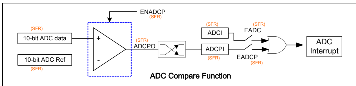
Figure 26-6: ADC Compare Function
