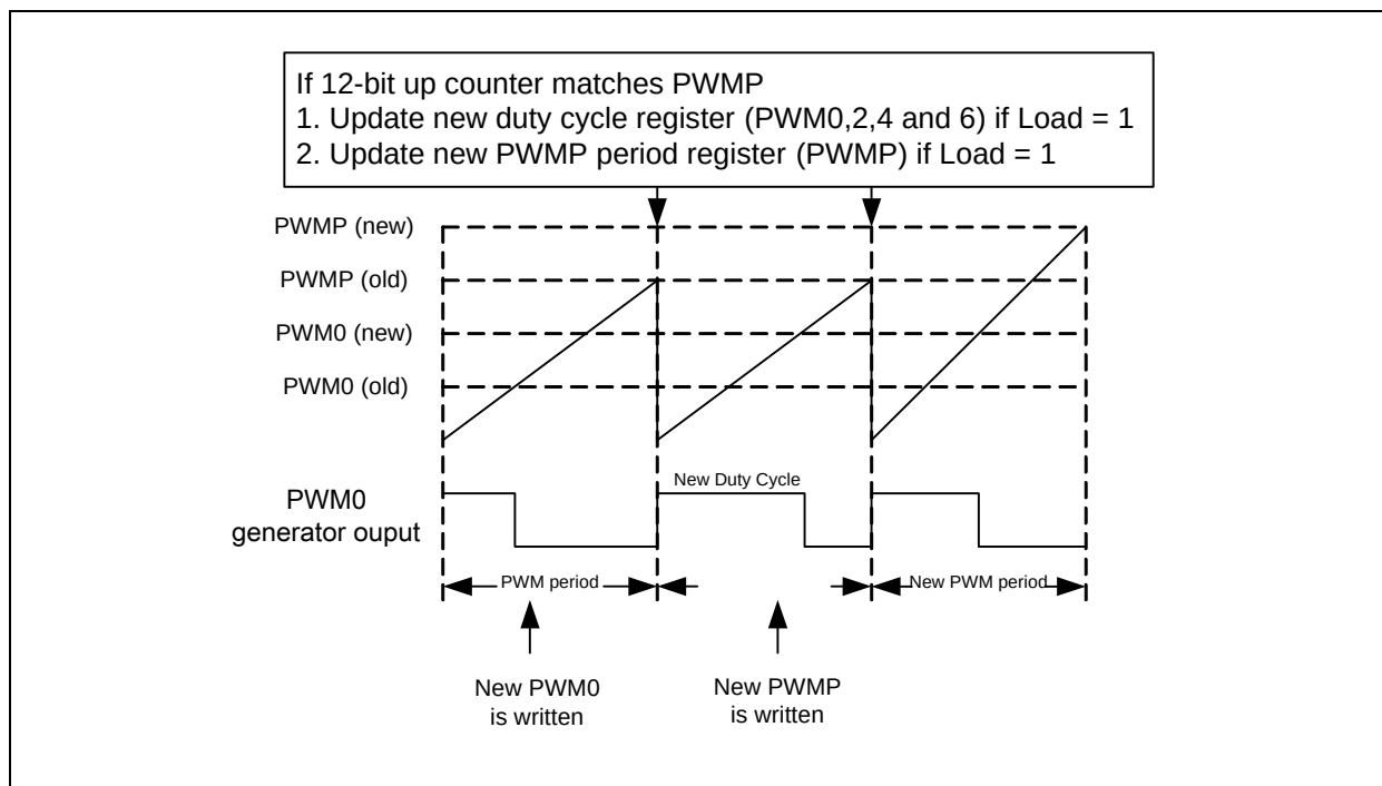
Figure 25-3: Edge-Aligned PWM
