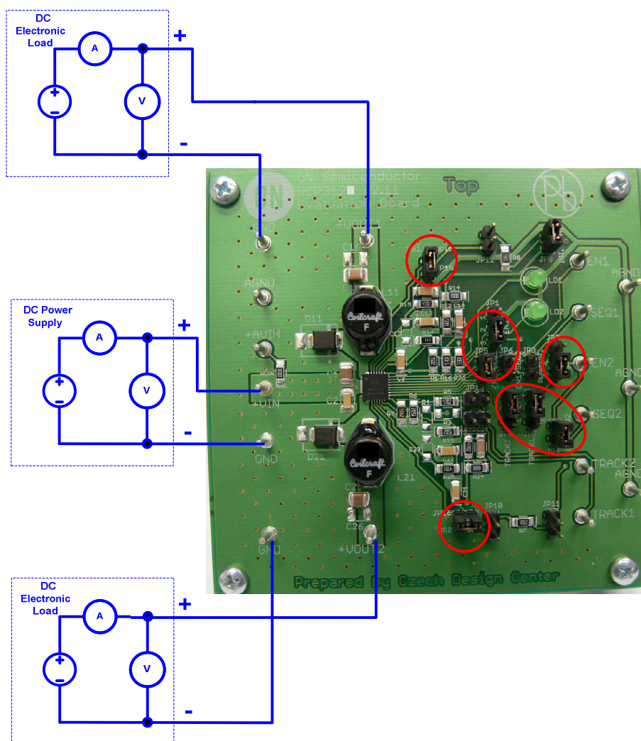
Figure 1. Test Setup
